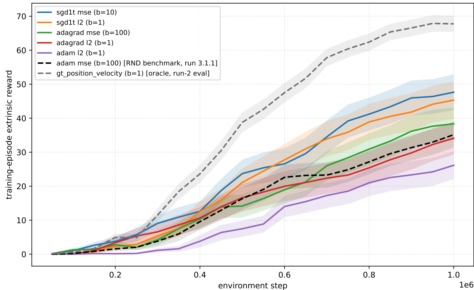
Run 3.2.1 best optimizer configs: training-episode reward vs step (mean \pm 1 SE over seeds, n \geq 10 )
