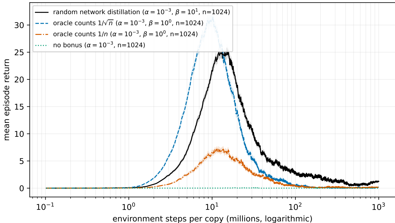
PointMaze large, no reset noise — each arm's best configuration, 1000M steps
