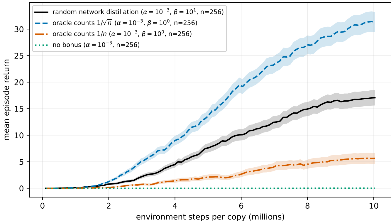
PointMaze large, no reset noise — best configuration of each arm
