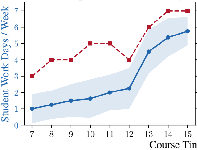
(a) w/o Speculative Scaffolding
