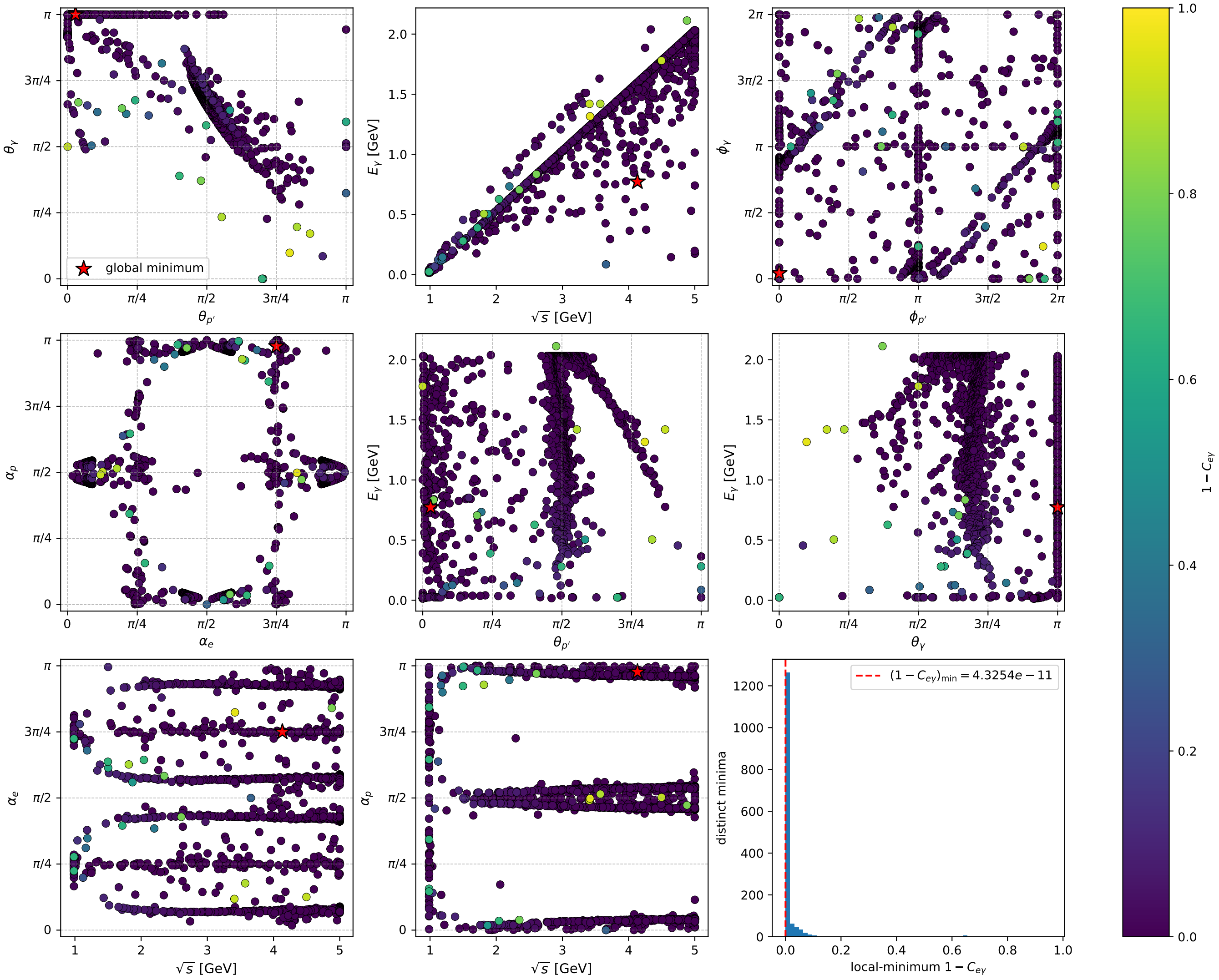
electron: all 1464 distinct gradient-search local minima of 1 - C_{ey}
