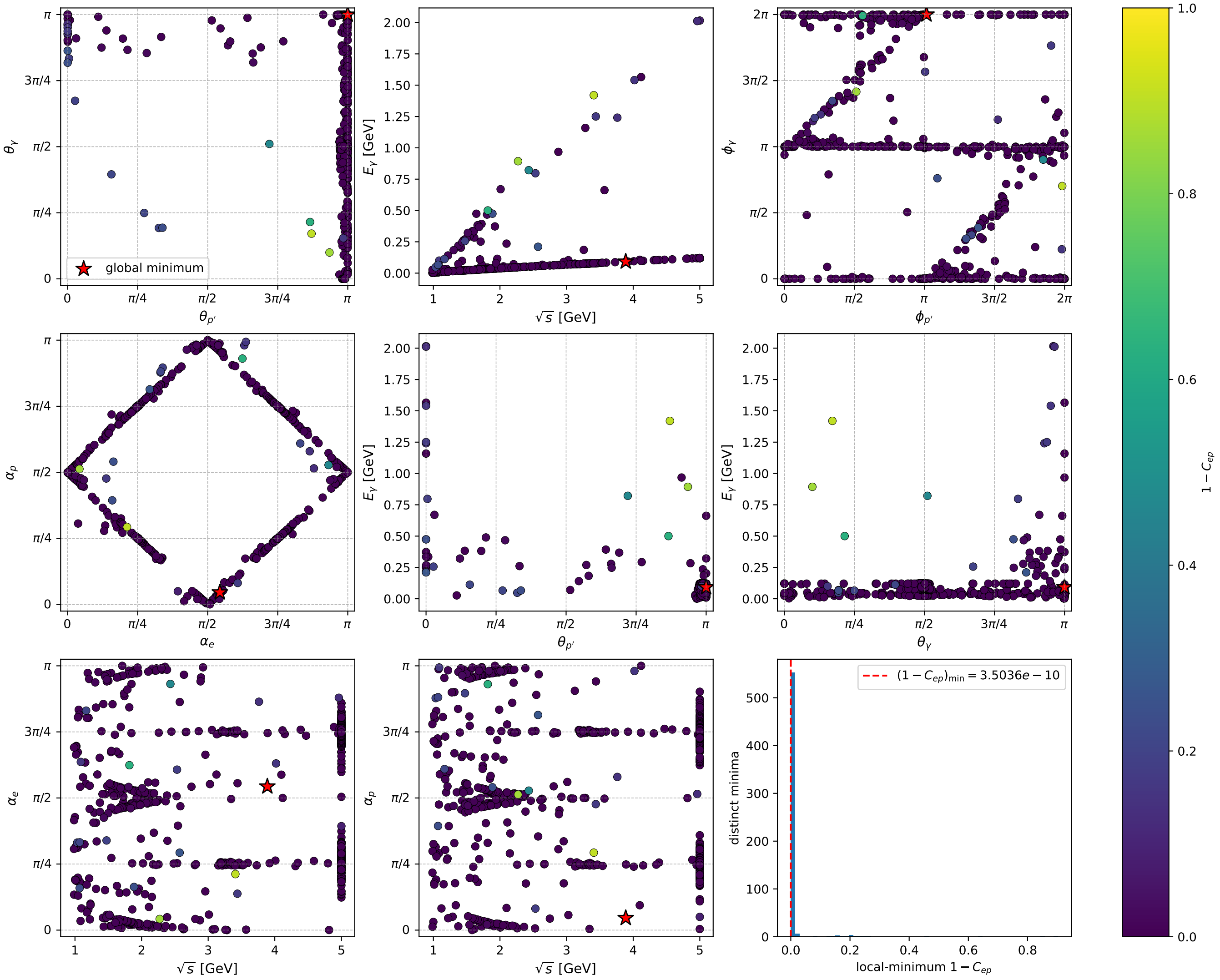
electron: all 577 distinct gradient-search local minima of 1 - C_{ep}
