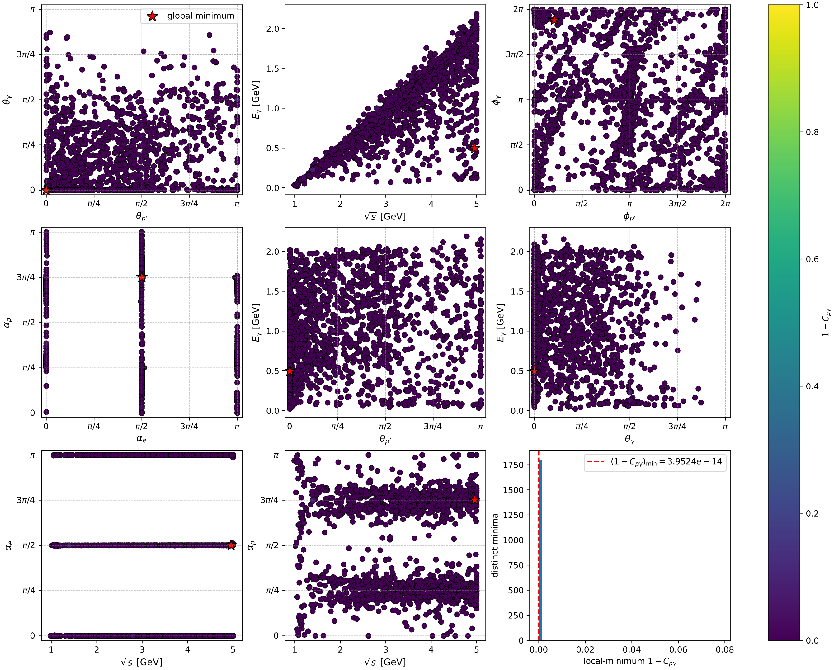
electron: all 1821 distinct gradient-search local minima of 1 - C_{p\gamma}
