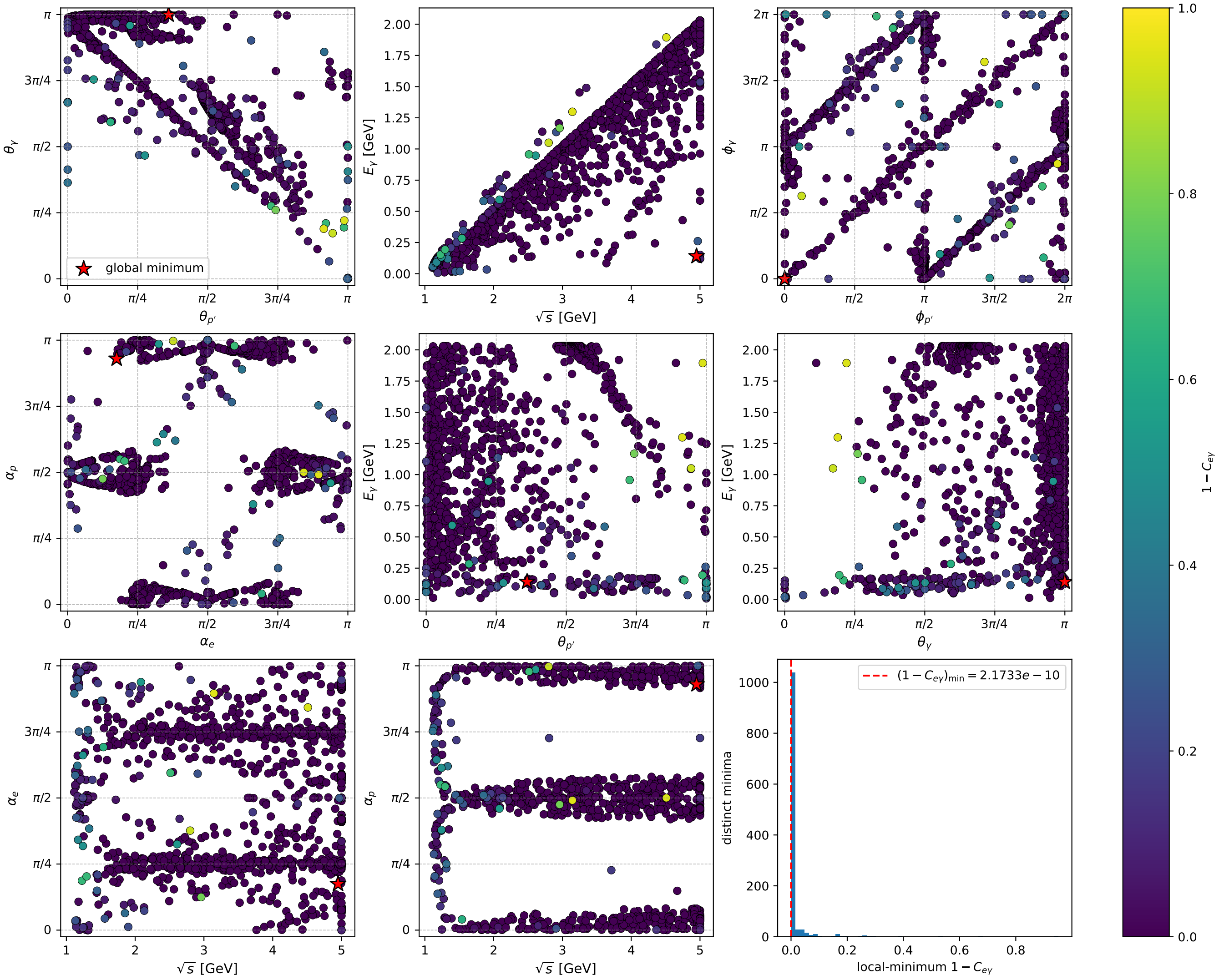
muon: all 1177 distinct gradient-search local minima of 1 - C_{ey}
