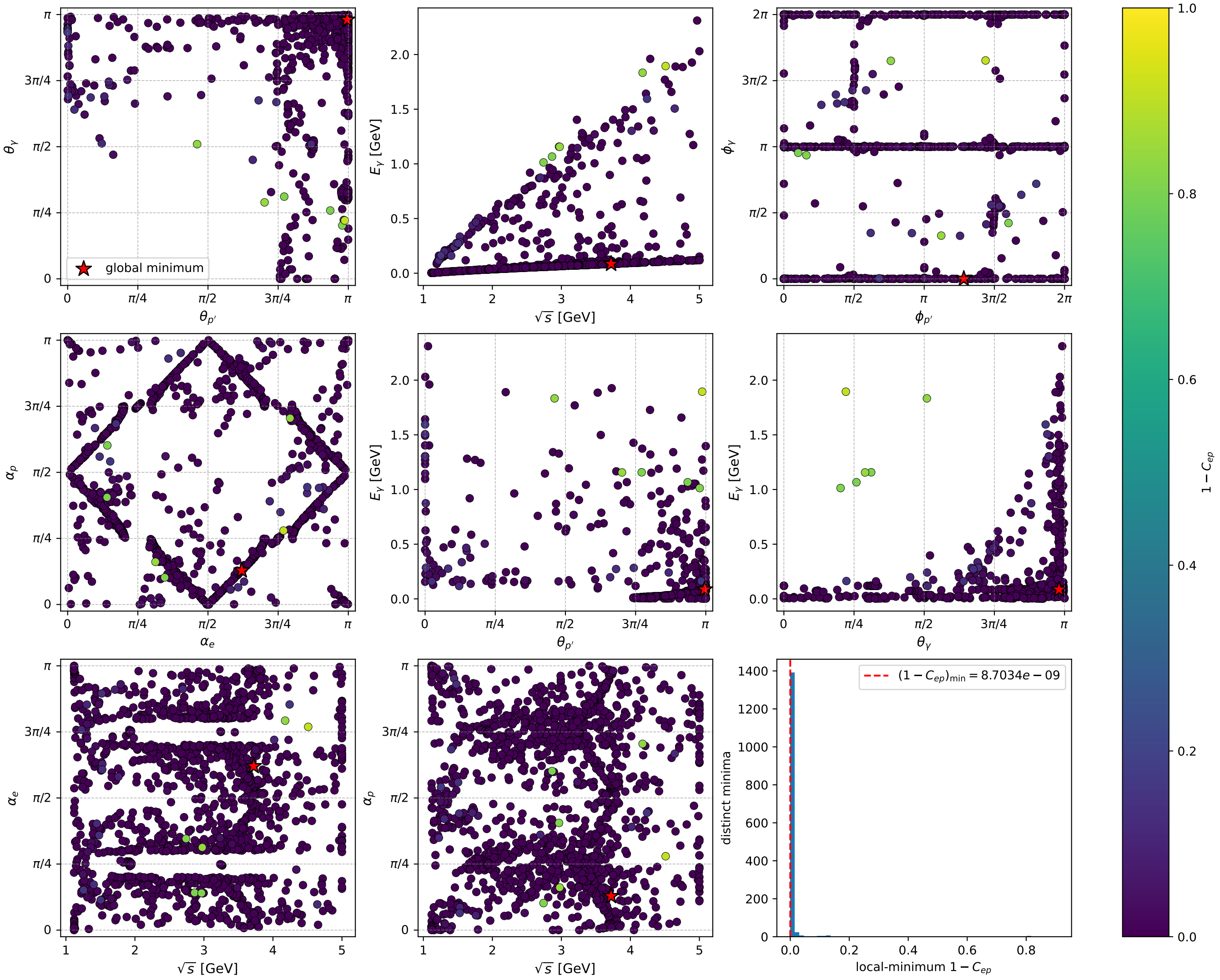
muon: all 1443 distinct gradient-search local minima of 1 - C_{ep}
