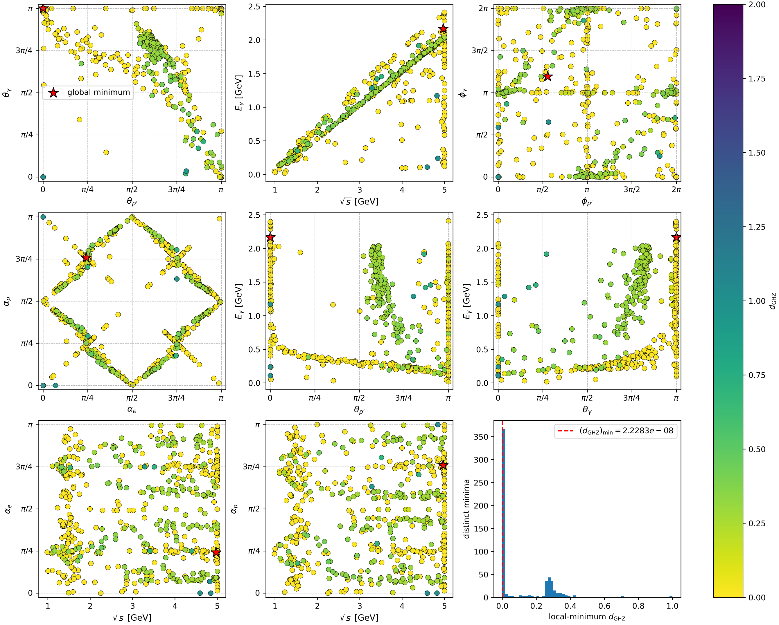
electron: all 579 distinct gradient-search local minima of d_{\text{GHZ}}
