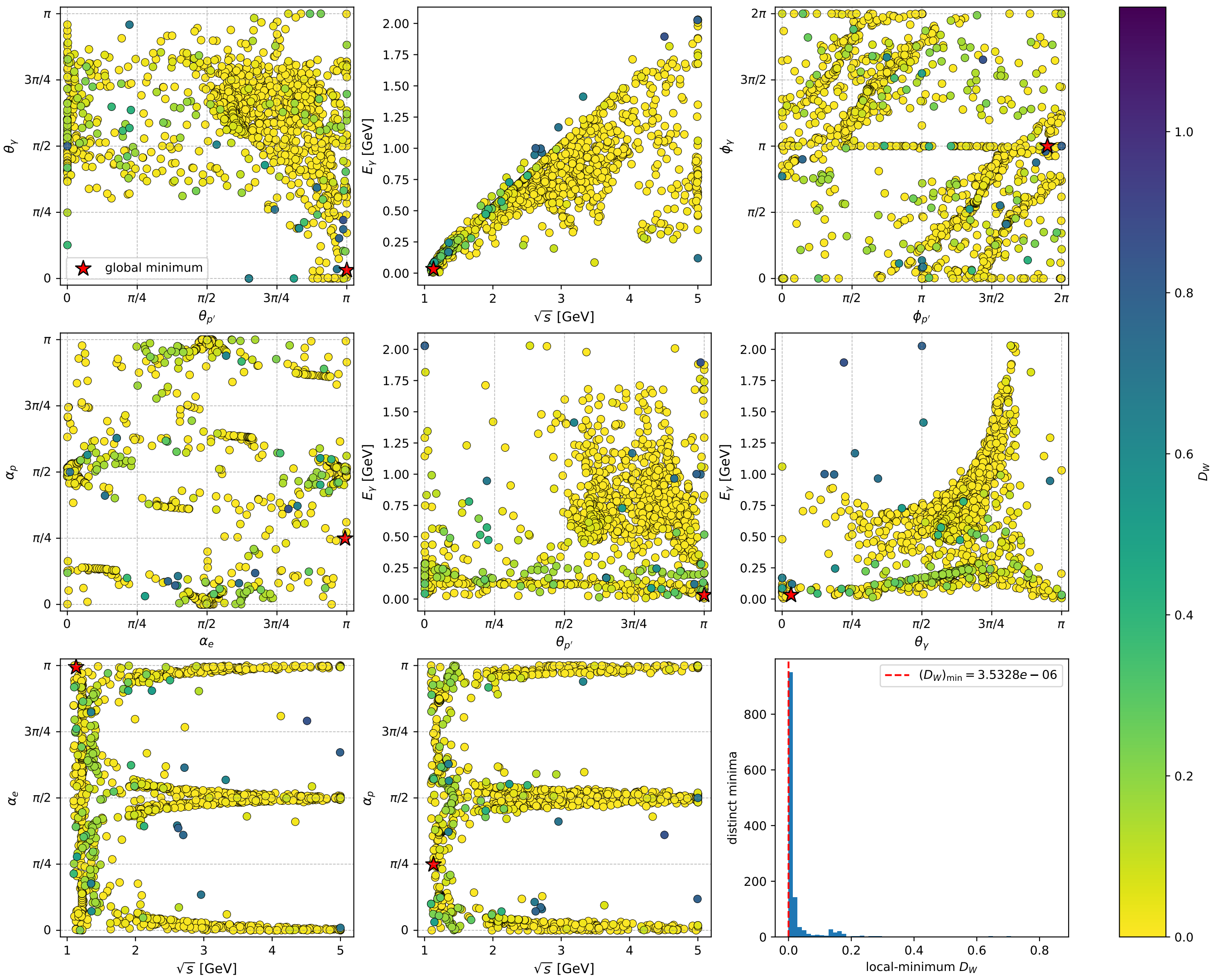
muon: all 1296 distinct gradient-search local minima of D_W
