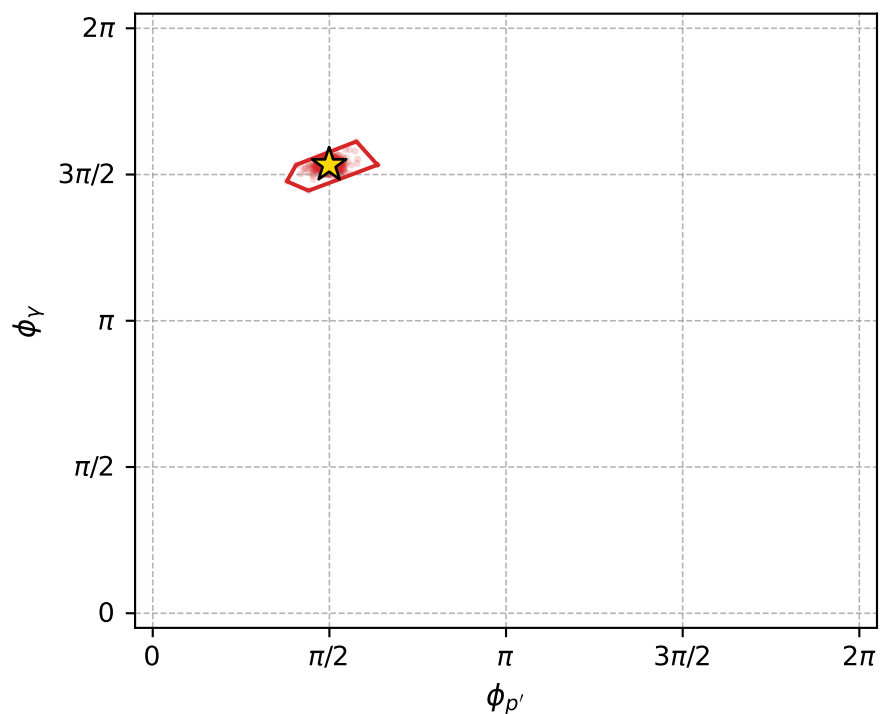
muon: polarization cluster P3, local minimum 726; pairwise projections of the 8D D_W = (D_W)_{\text{local}} + 0.05 contour
