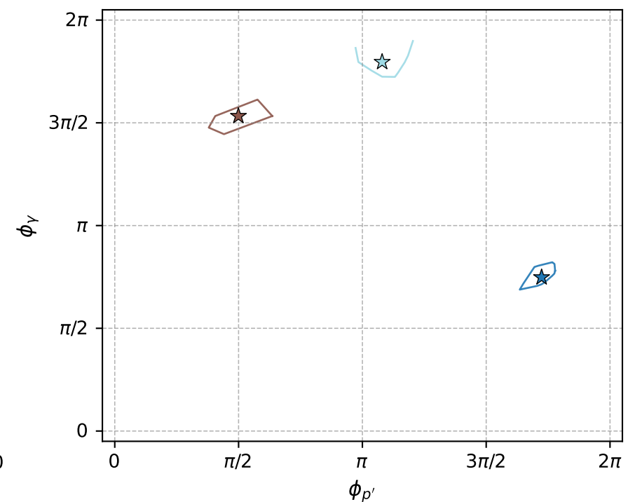
muon: polarization cluster P3; all local-minimum configurations and pairwise projections of their 8D contours
