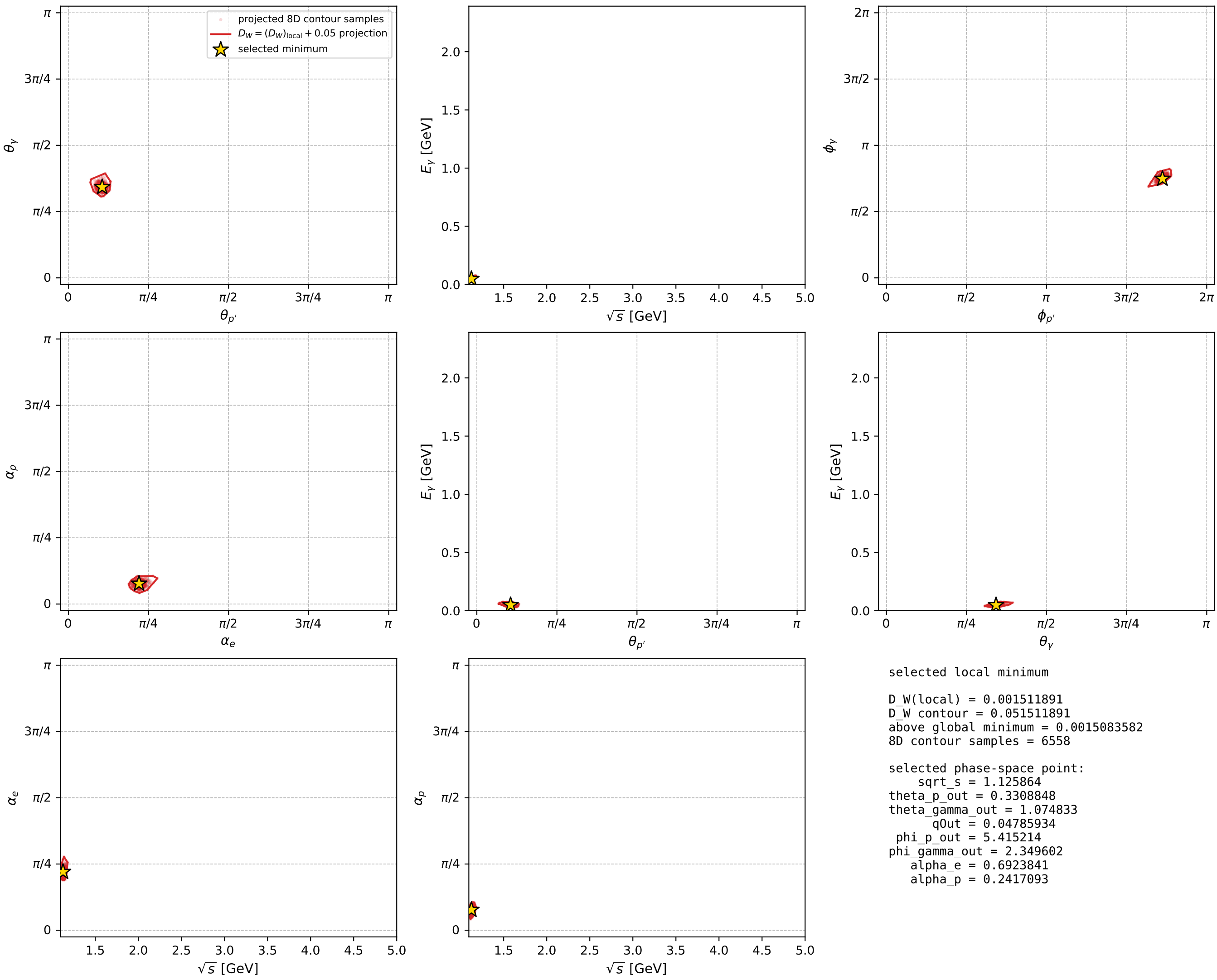
muon: polarization cluster P3, local minimum 584; pairwise projections of the 8D D_W = (D_W)_{\text{local}} + 0.05 contour
