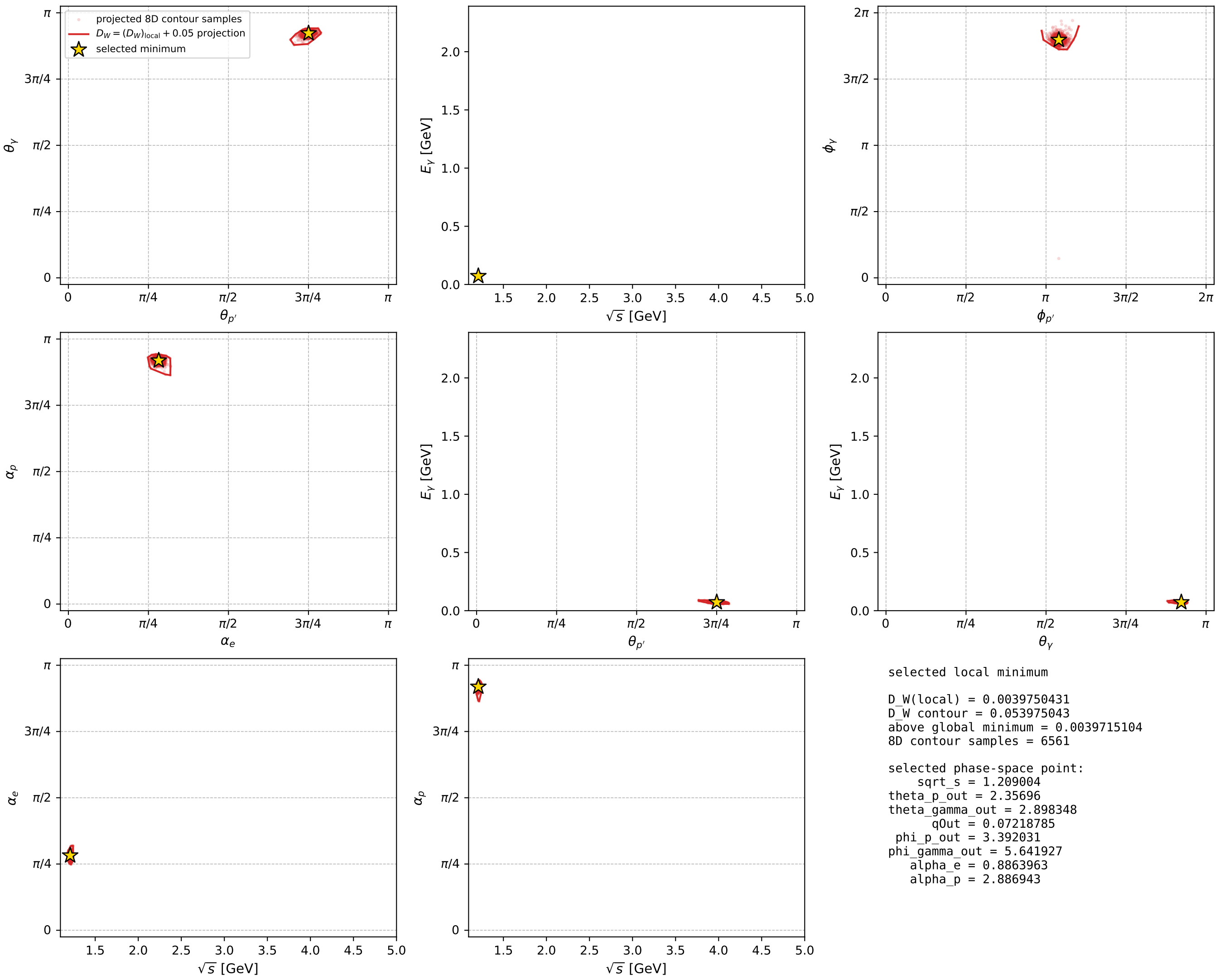
muon: polarization cluster P3, local minimum 734; pairwise projections of the 8D D_W = (D_W)_{\text{local}} + 0.05 contour
