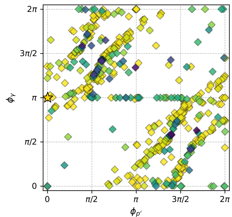
muon: polarization cluster P4; all member minima in phase space
