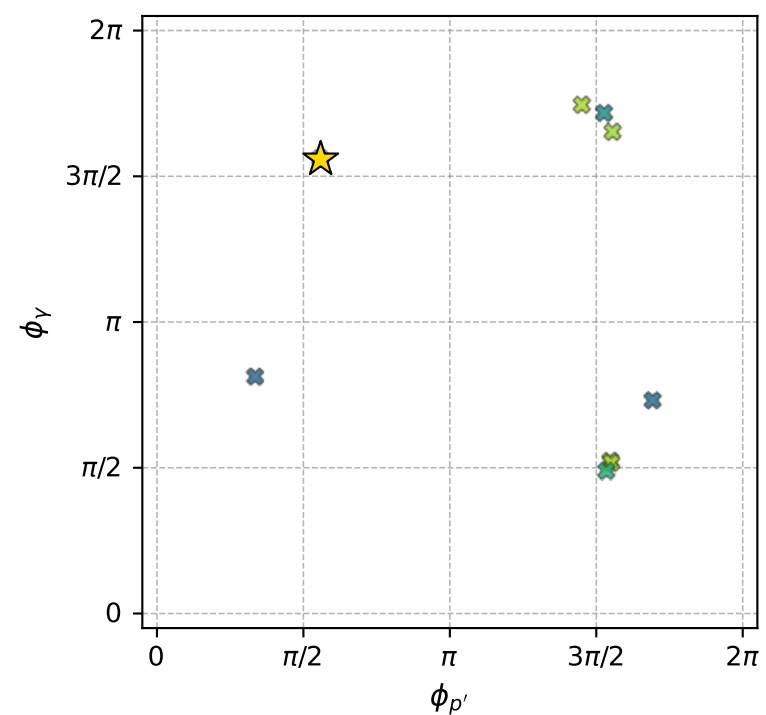
muon: polarization cluster P6; all member minima in phase space
