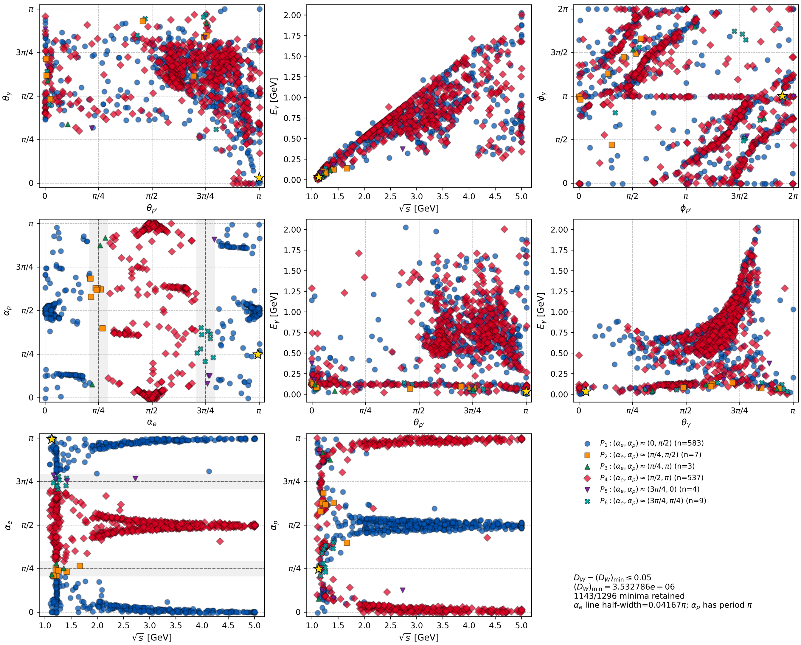
muon: low- D_W phase space colored by 6 major polarization configurations
