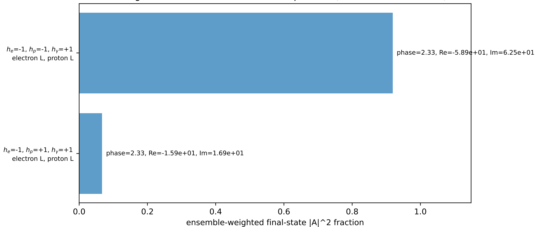
Leading initial-ensemble/final-state components (N=2, retained=98.6%)
