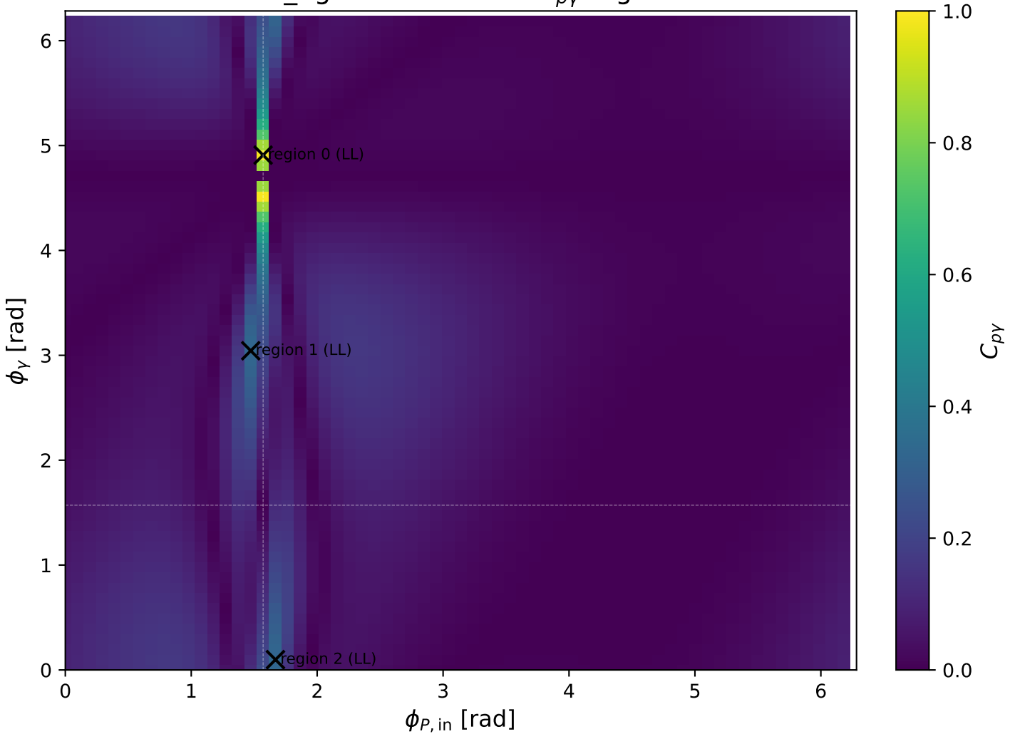
mid_Egamma LL: max C_{p\gamma} regions
