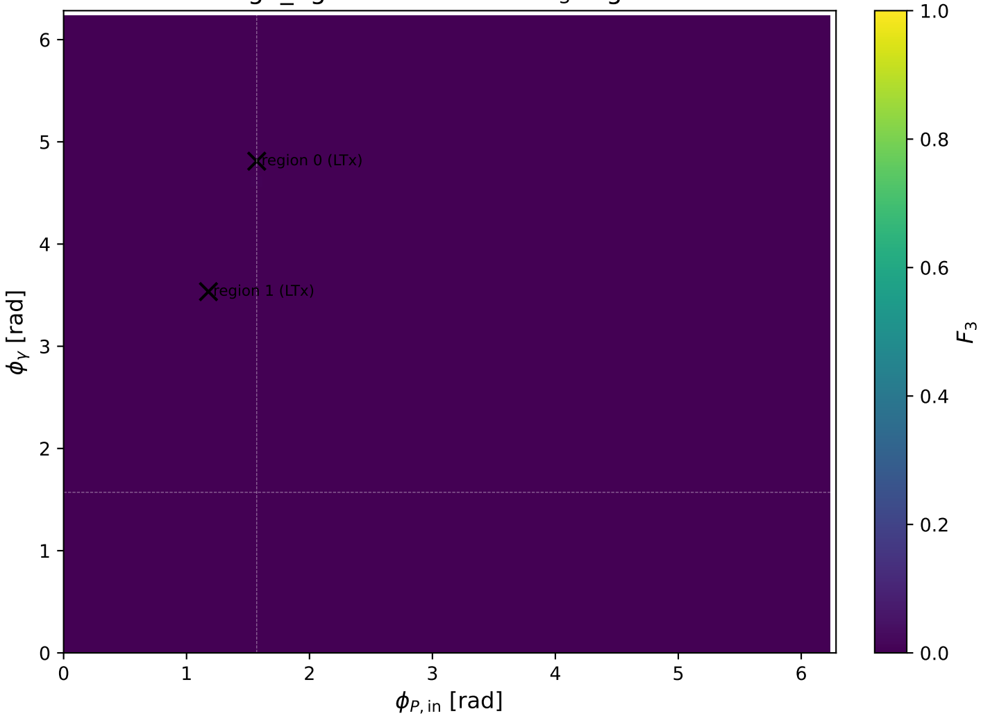
high_Egamma LTx: max F_3 regions
