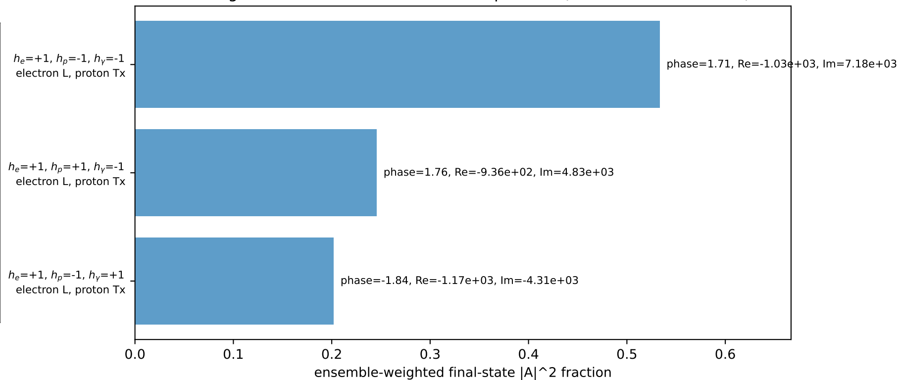
Leading initial-ensemble/final-state components (N=3, retained=98.1%)
