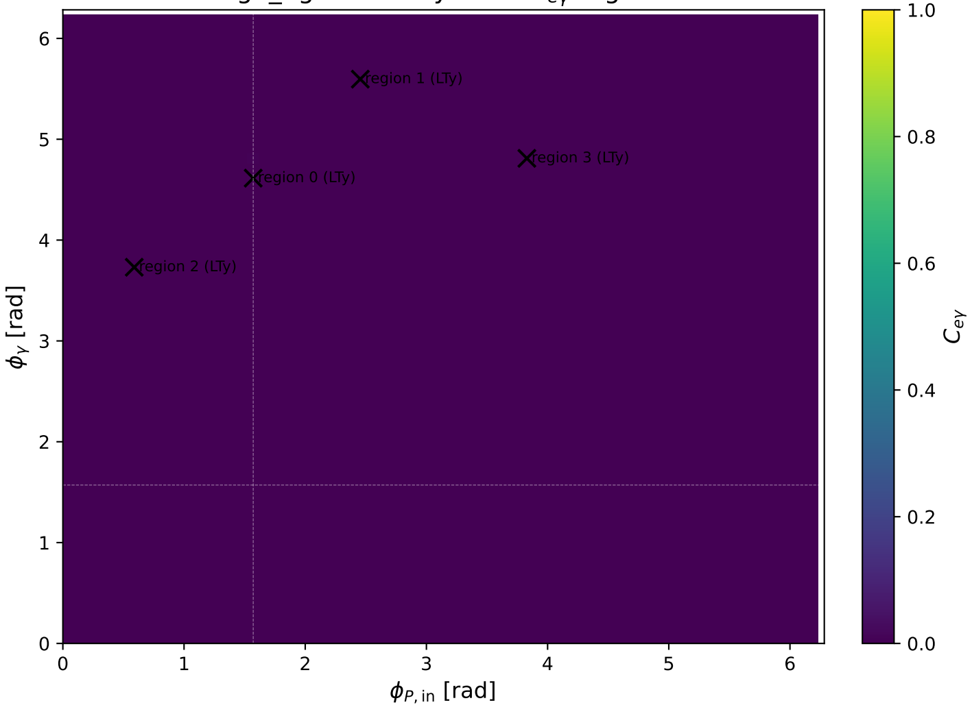
high_Egamma LTy: max C_{e\gamma} regions
