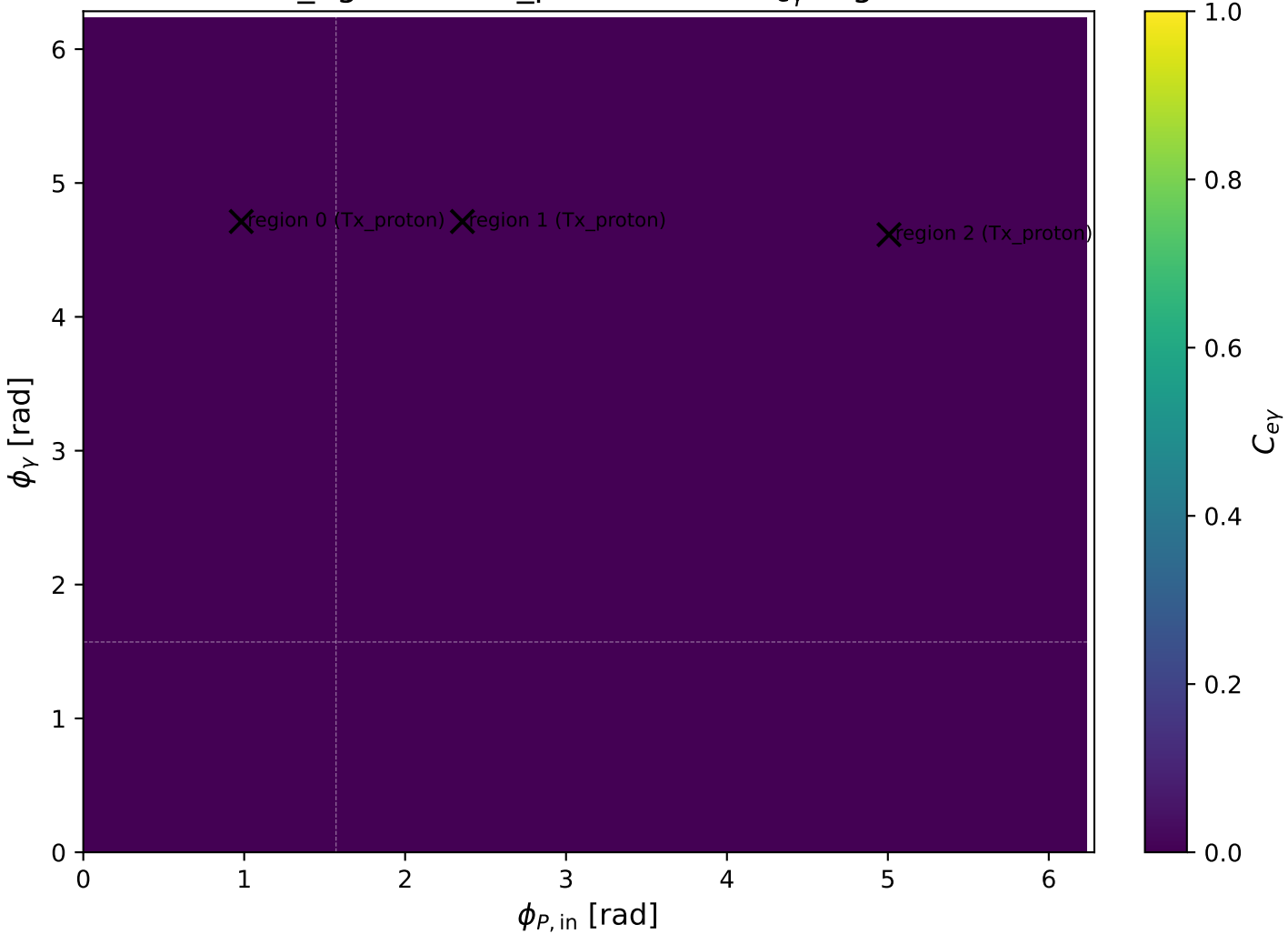
mid_Egamma Tx_proton: max C_{e\gamma} regions
