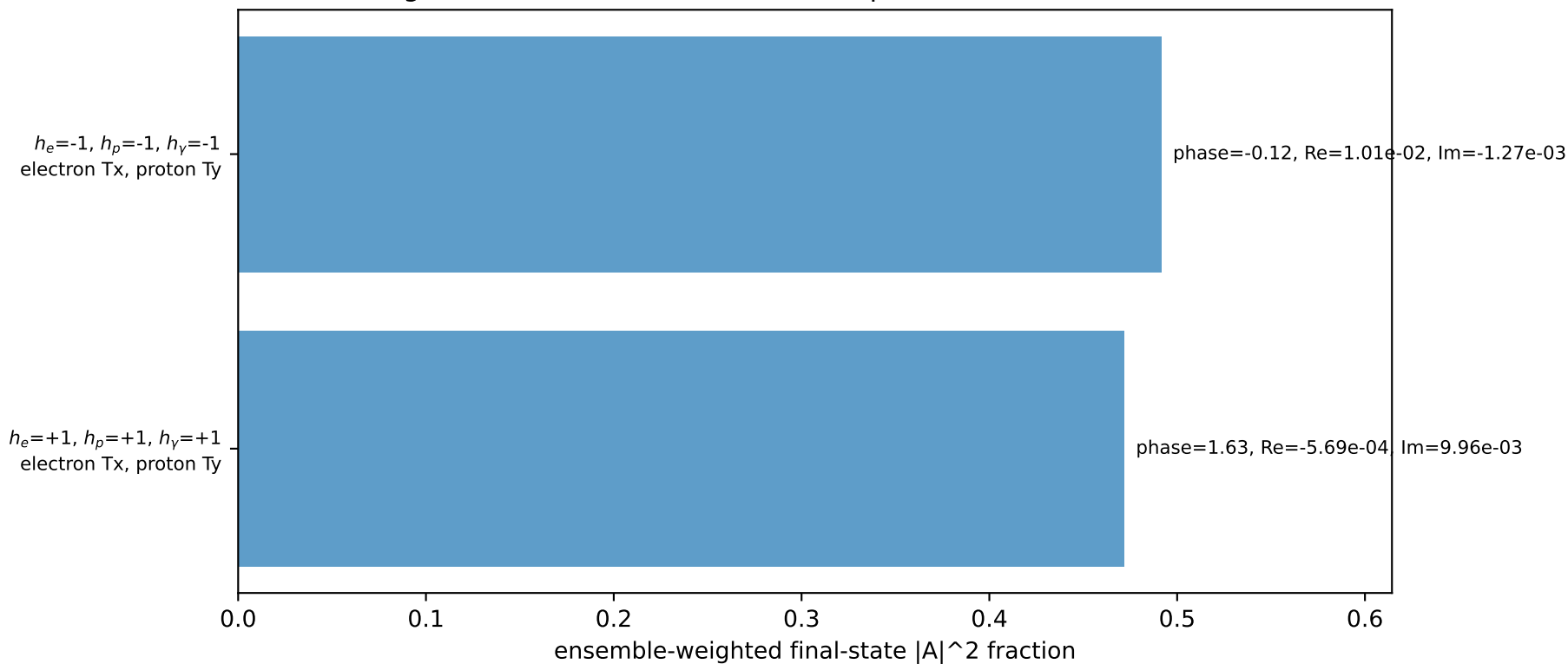
Leading initial-ensemble/final-state components (N=2, retained=96.3%)
