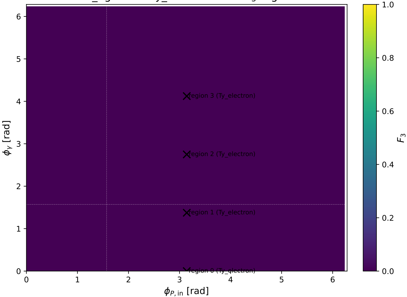
low_Egamma Ty_electron: max F_3 regions
