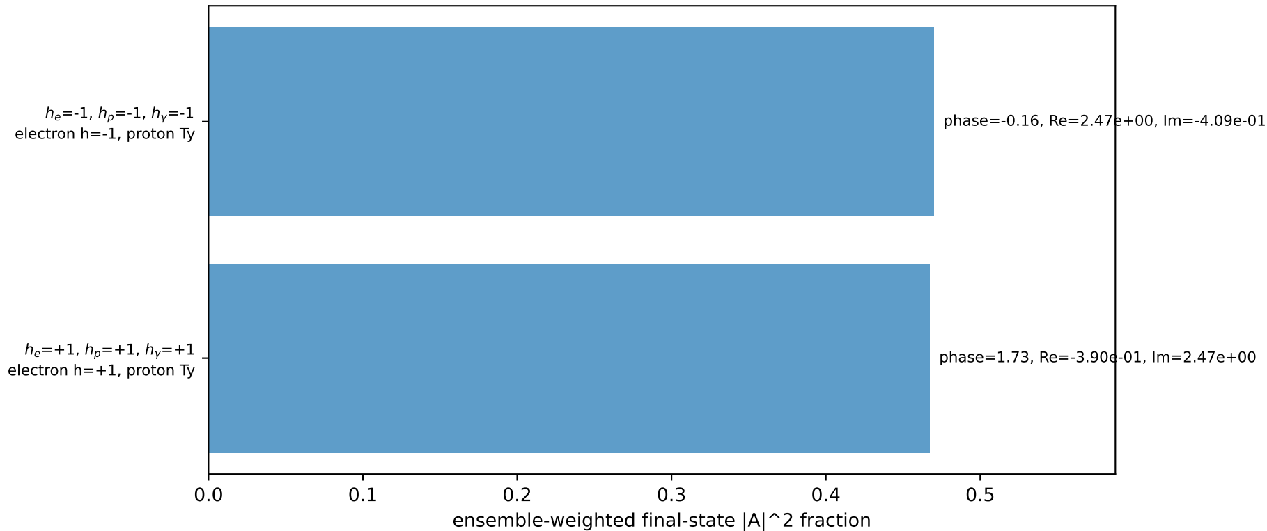
Leading initial-ensemble/final-state components (N=2, retained=93.7%)
