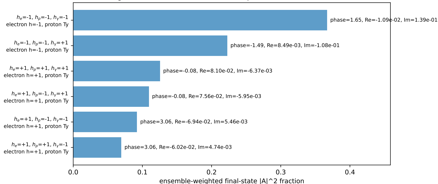
Leading initial-ensemble/final-state components (N=6, retained=98.5%)
