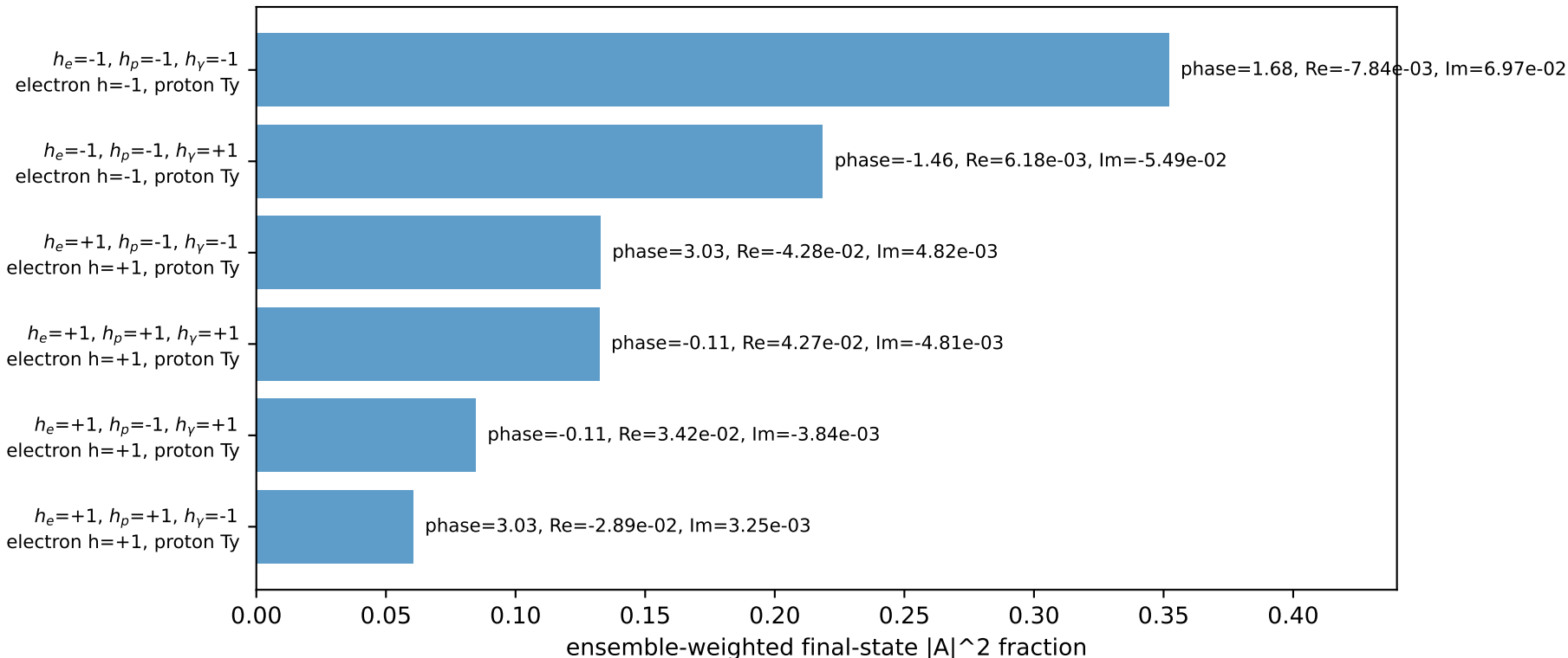
Leading initial-ensemble/final-state components (N=6, retained=98.1%)
