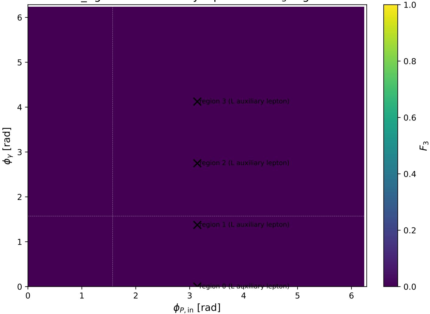
low_Egamma L auxiliary lepton: max F_3 regions
