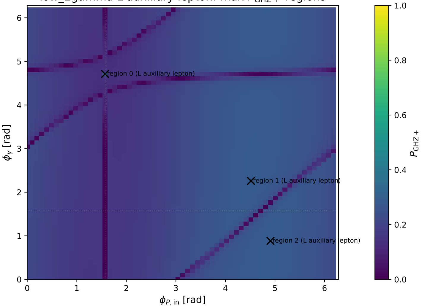
low_Egamma L auxiliary lepton: max P_{\text{GHZ}+} regions
