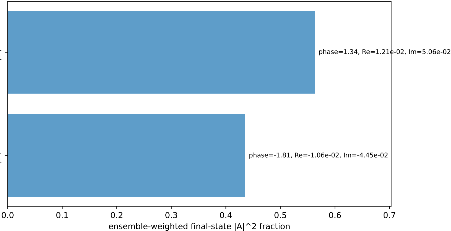
Leading initial-ensemble/final-state components (N=2, retained=99.7%)
