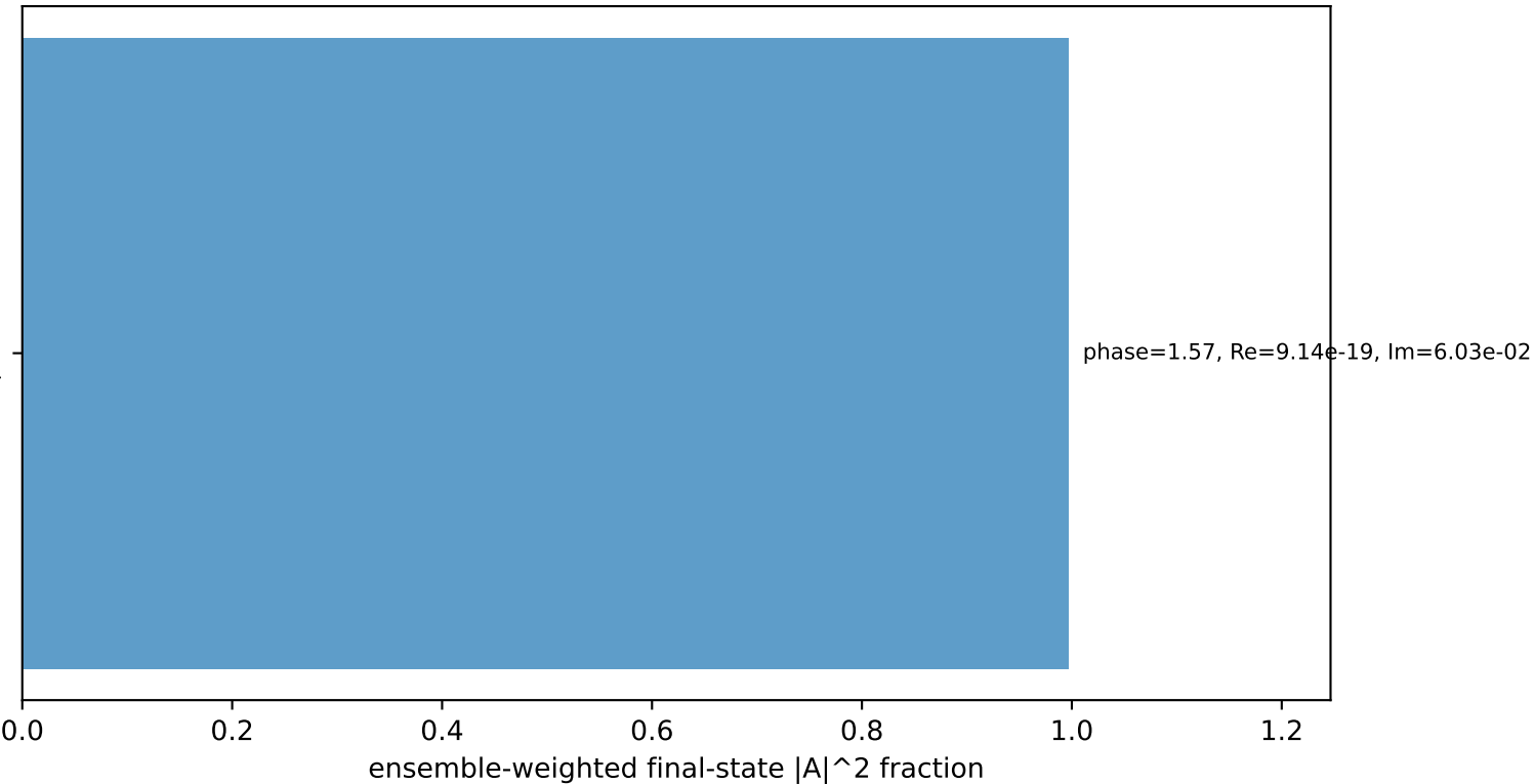
Leading initial-ensemble/final-state components (N=1, retained=99.7%)
