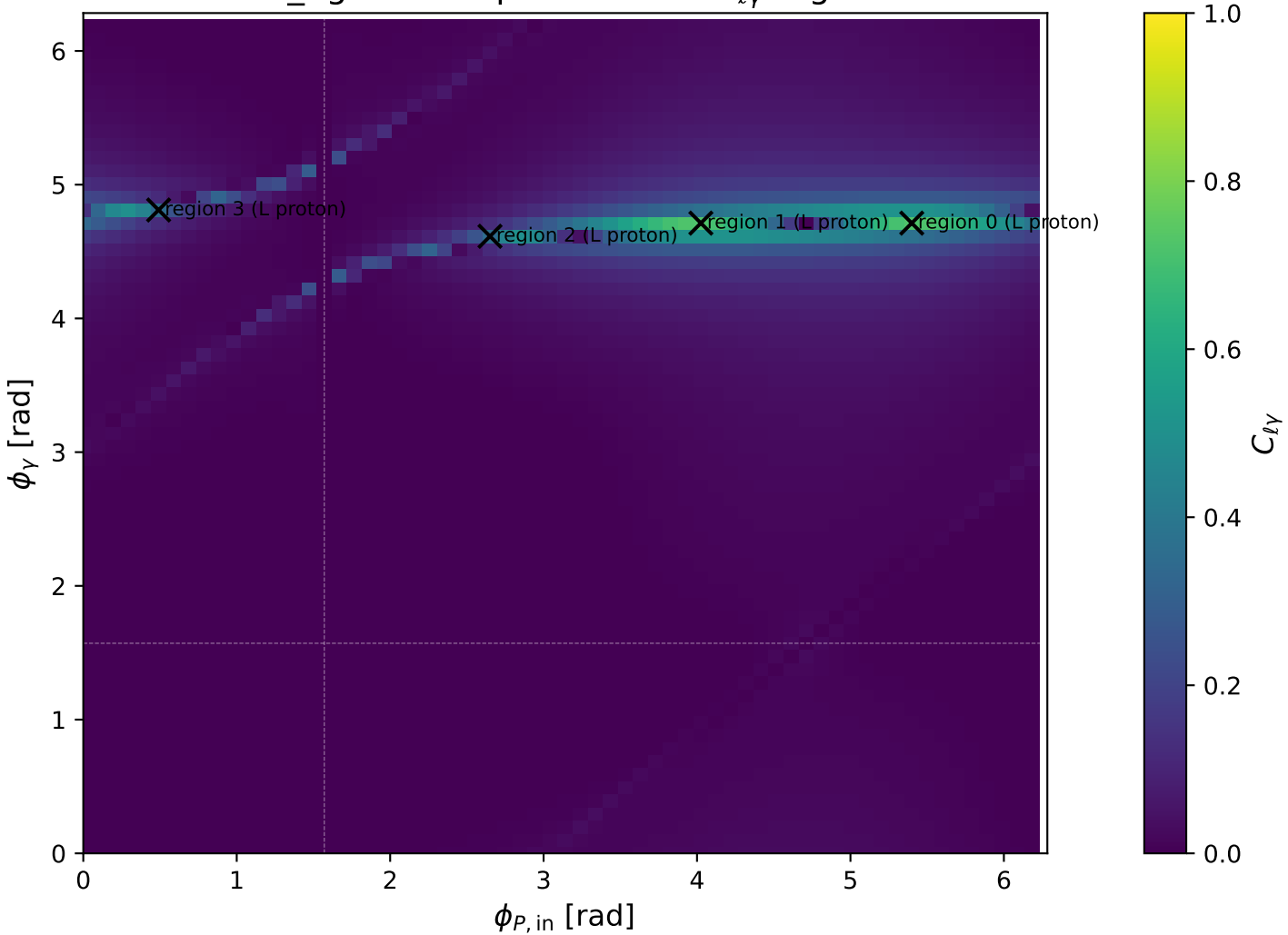
low_Egamma L proton: max C_{\ell\gamma} regions
