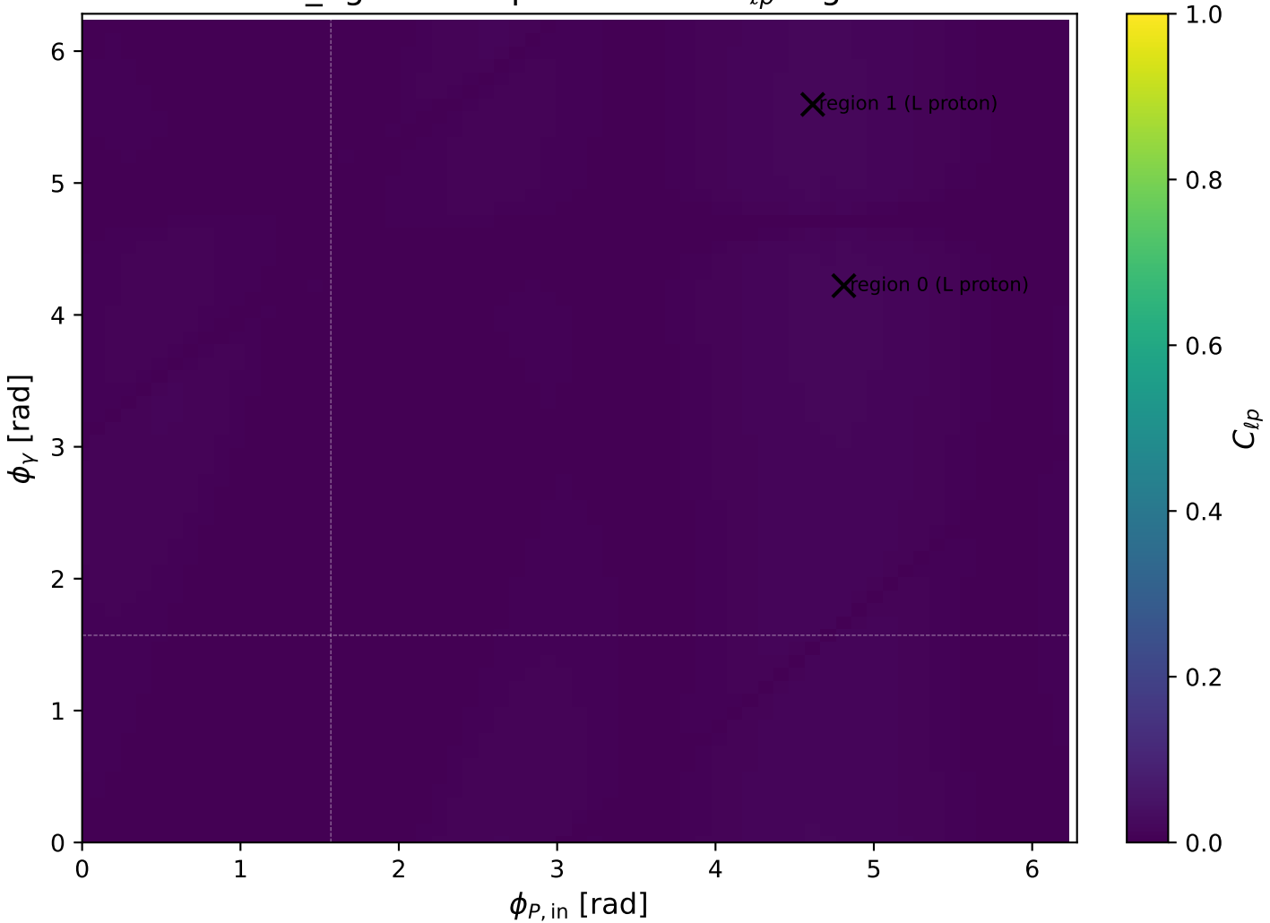
low_Egamma L proton: max C_{lp} regions
