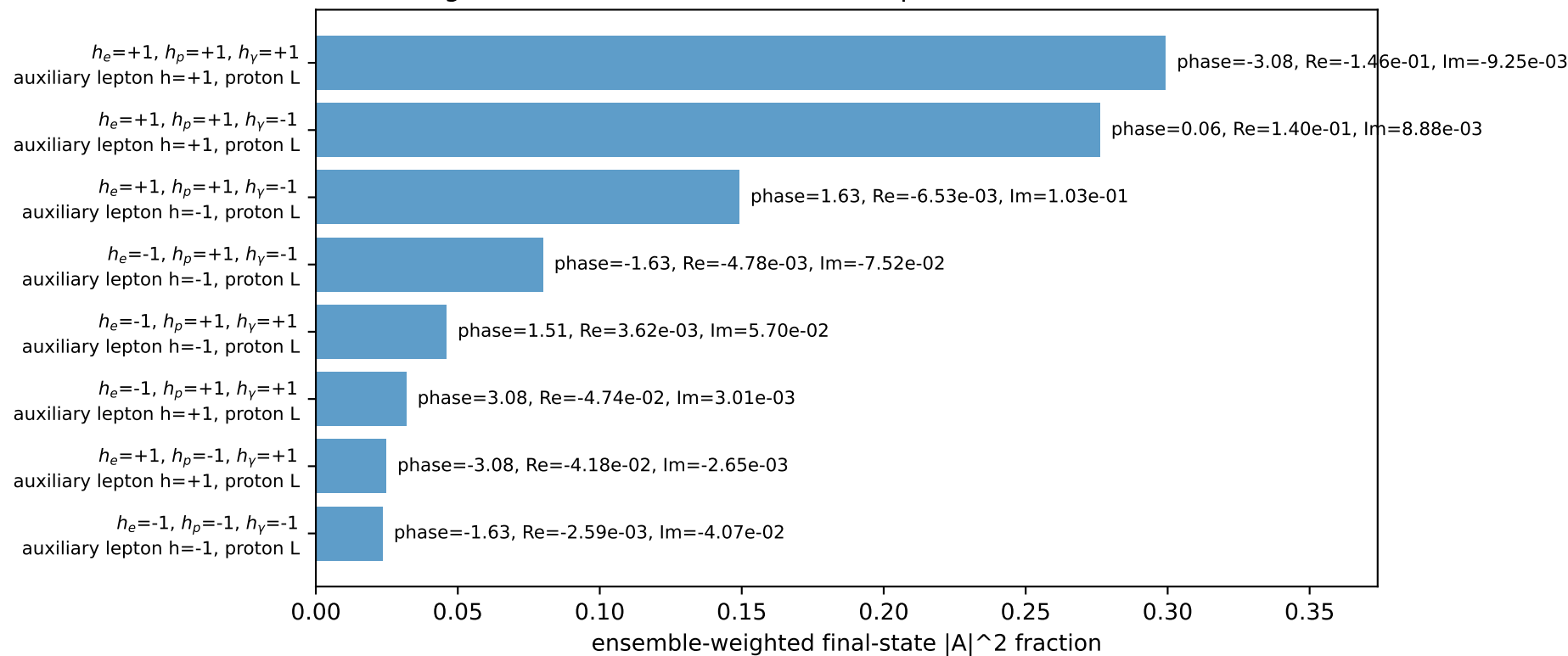
Leading initial-ensemble/final-state components (N=8, retained=93.0%)
