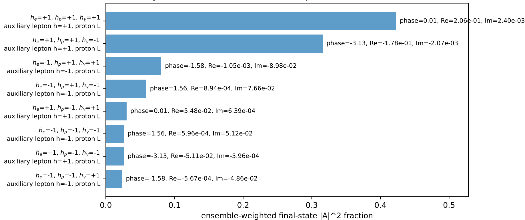
Leading initial-ensemble/final-state components (N=8, retained=98.3%)
