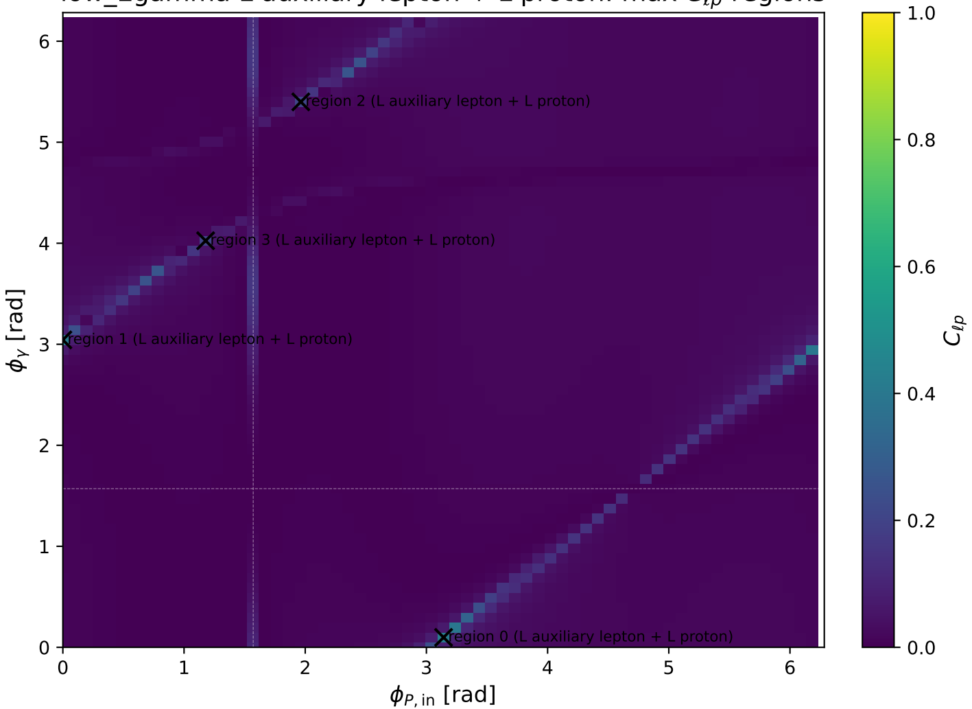
low_Egamma L auxiliary lepton + L proton: max C_{lp} regions
