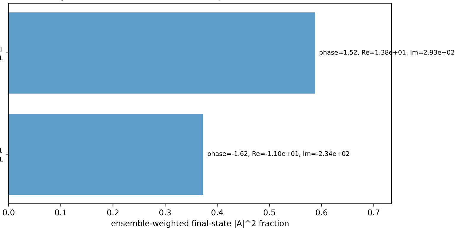
Leading initial-ensemble/final-state components (N=2, retained=96.0%)
