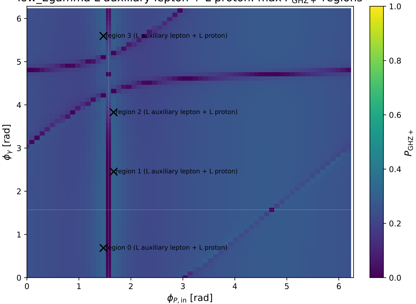
low_Egamma L auxiliary lepton + L proton: max P_{\text{GHZ}+} regions
