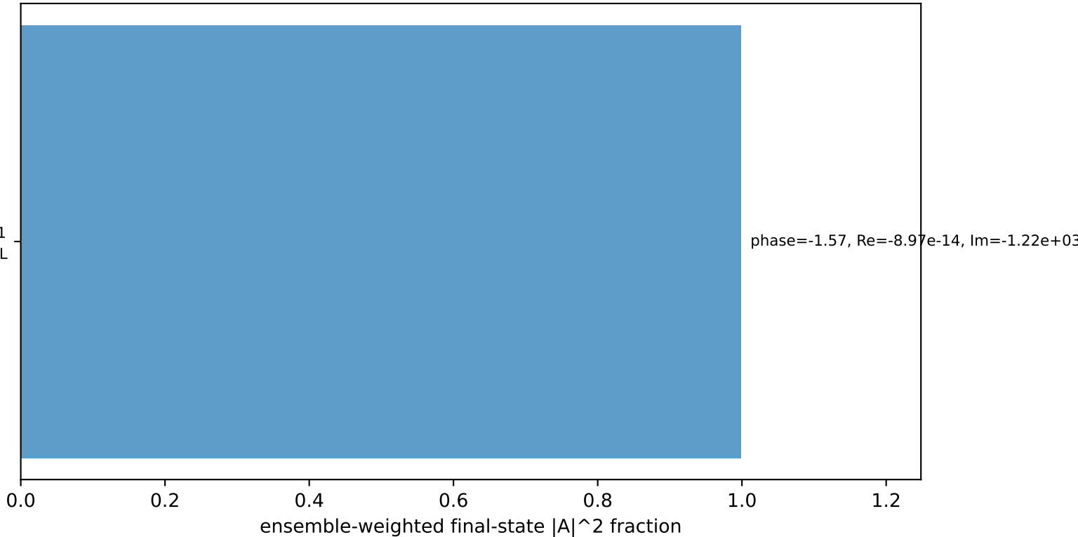
Leading initial-ensemble/final-state components (N=1, retained=99.9%)
