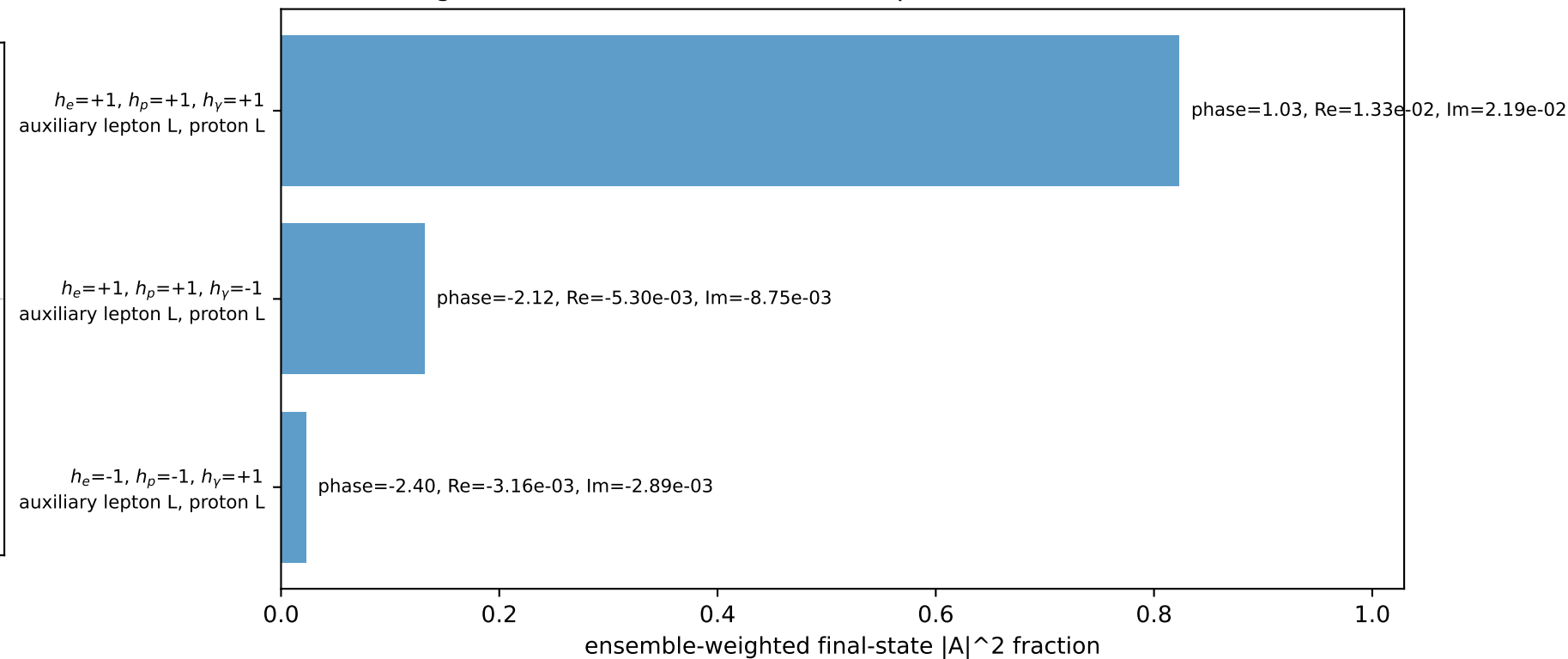
Leading initial-ensemble/final-state components (N=3, retained=97.8%)
