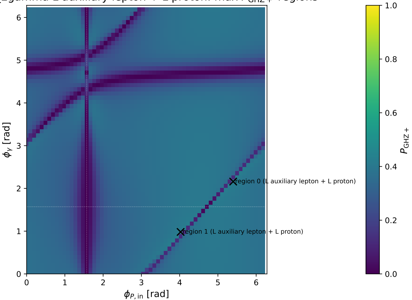
[Egamma L auxiliary lepton + L proton: max P_{\text{GHZ}} + regions
