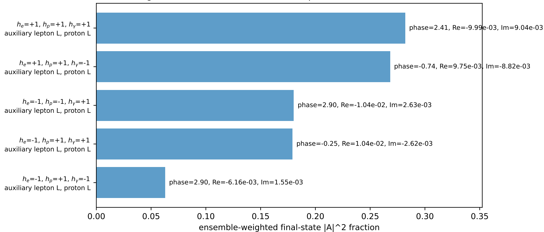
Leading initial-ensemble/final-state components (N=5, retained=97.2%)
