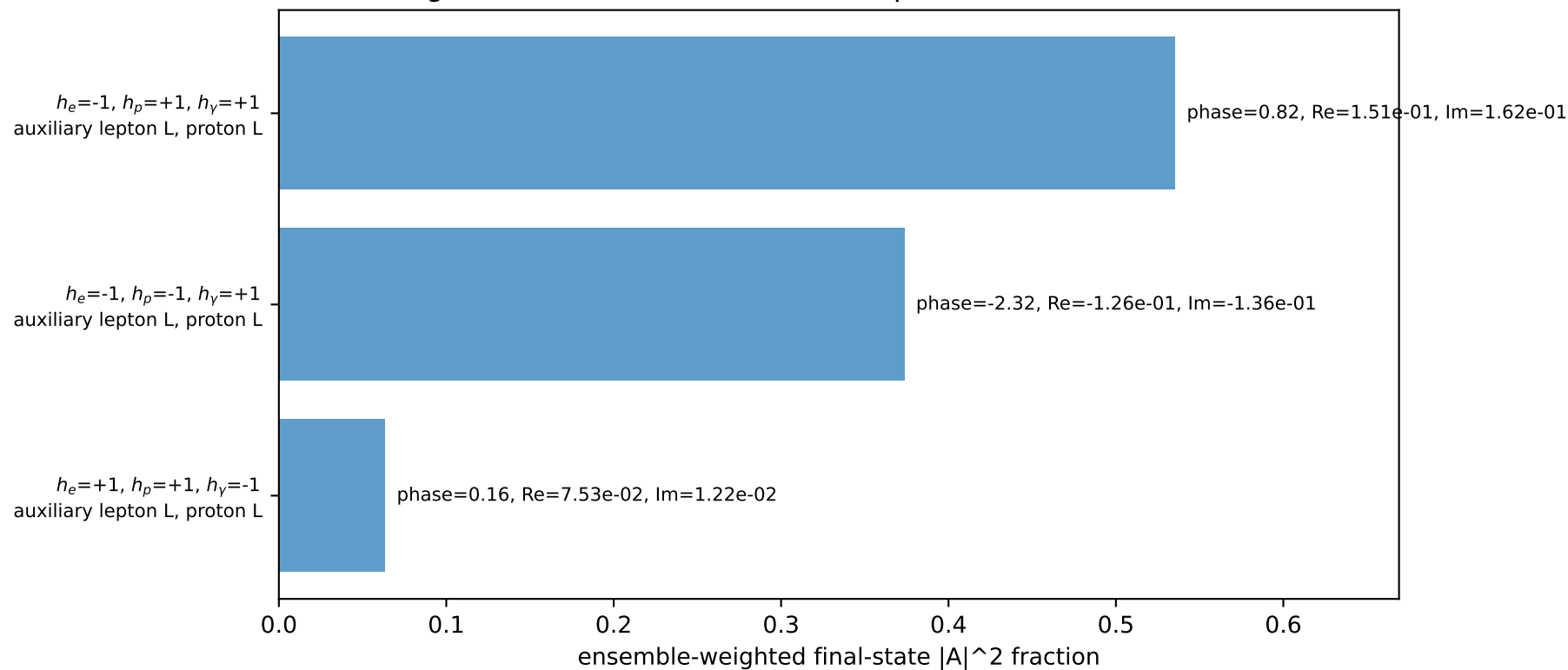
Leading initial-ensemble/final-state components (N=3, retained=97.2%)
