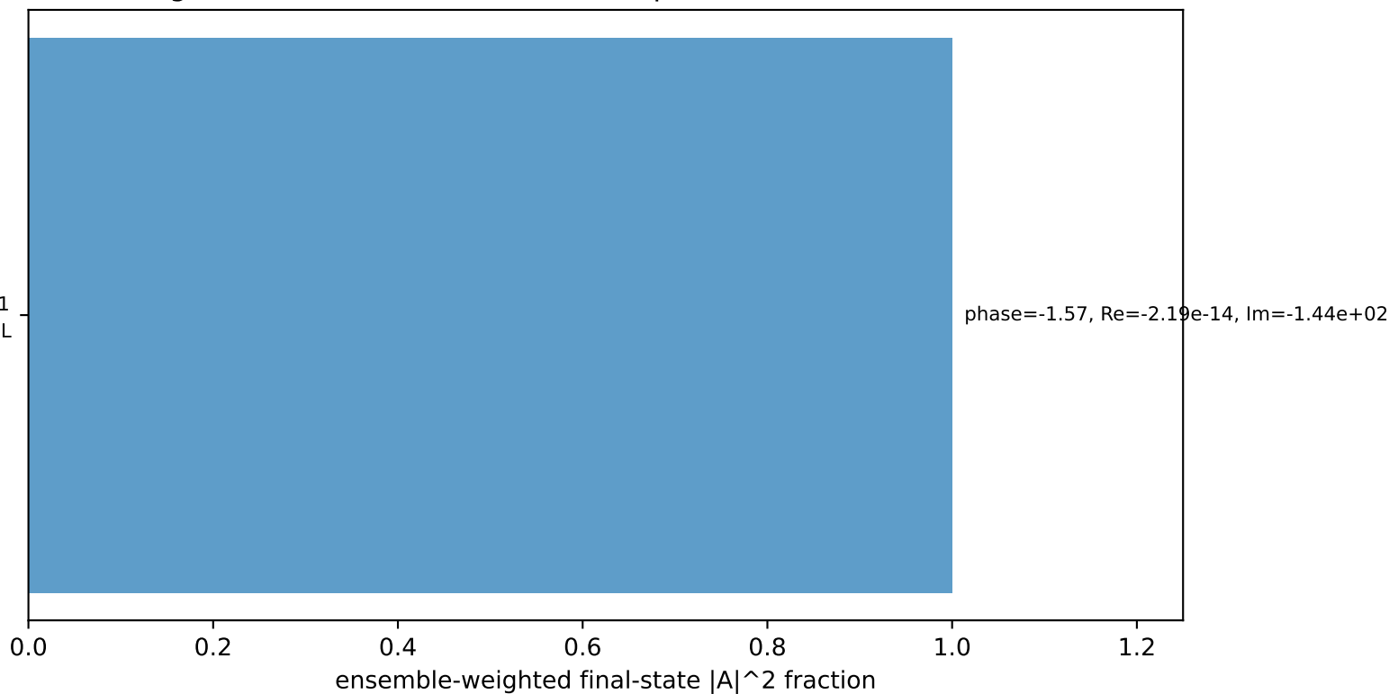
Leading initial-ensemble/final-state components (N=1, retained=100.0%)
