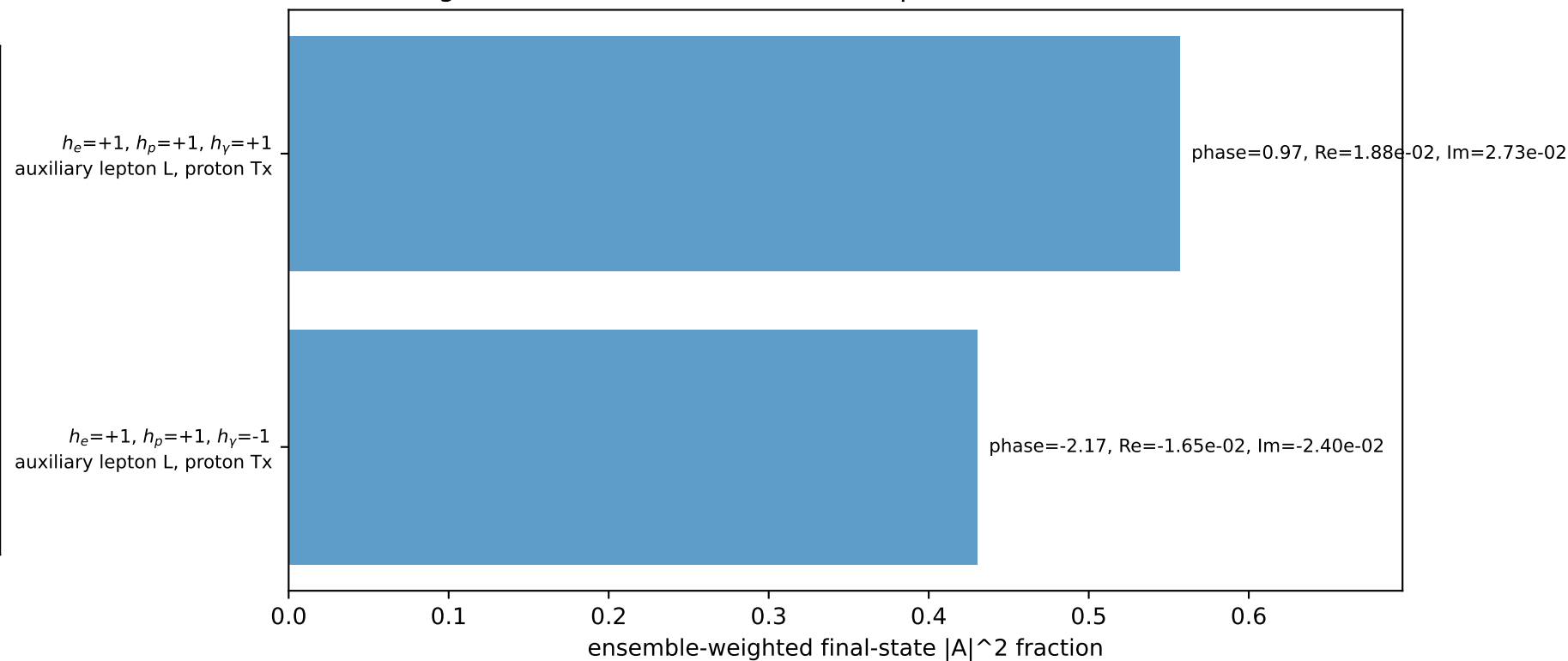
Leading initial-ensemble/final-state components (N=2, retained=98.7%)
