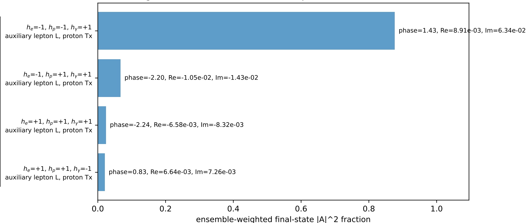
Leading initial-ensemble/final-state components (N=4, retained=98.8%)
