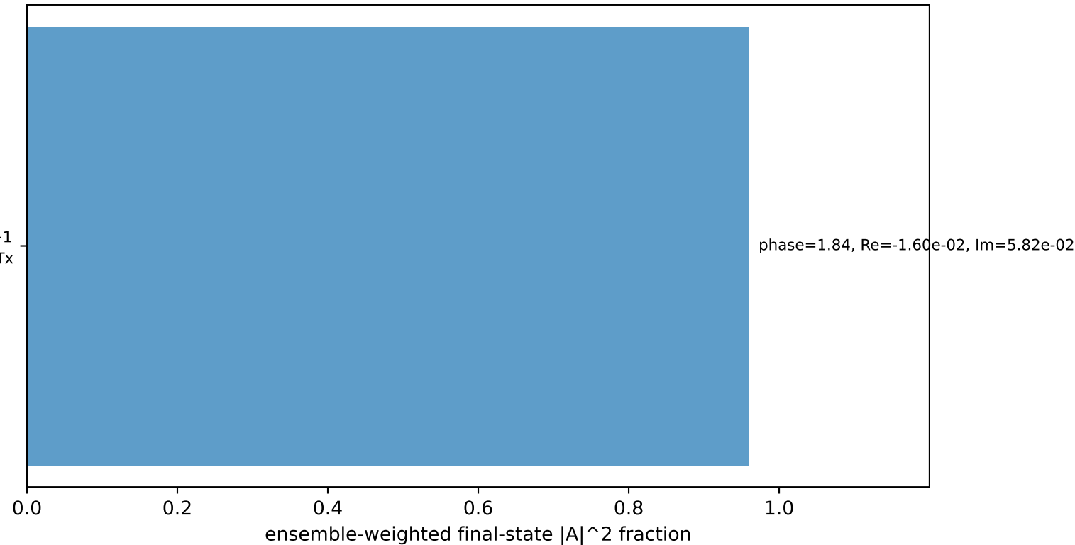
Leading initial-ensemble/final-state components (N=1, retained=96.0%)
