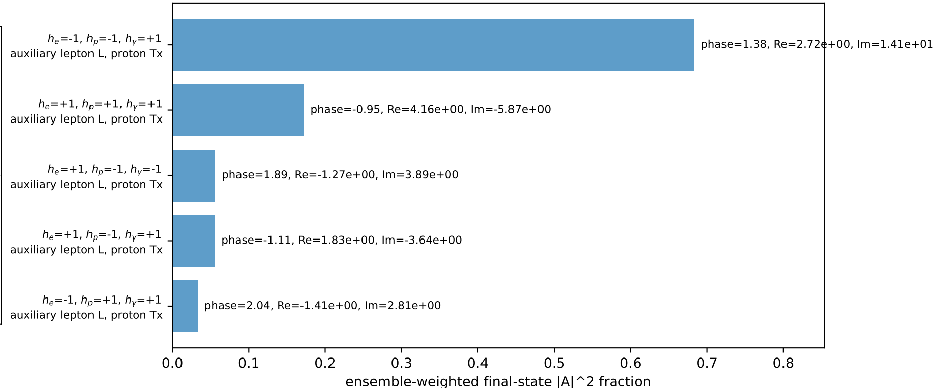
Leading initial-ensemble/final-state components (N=5, retained=99.8%)
