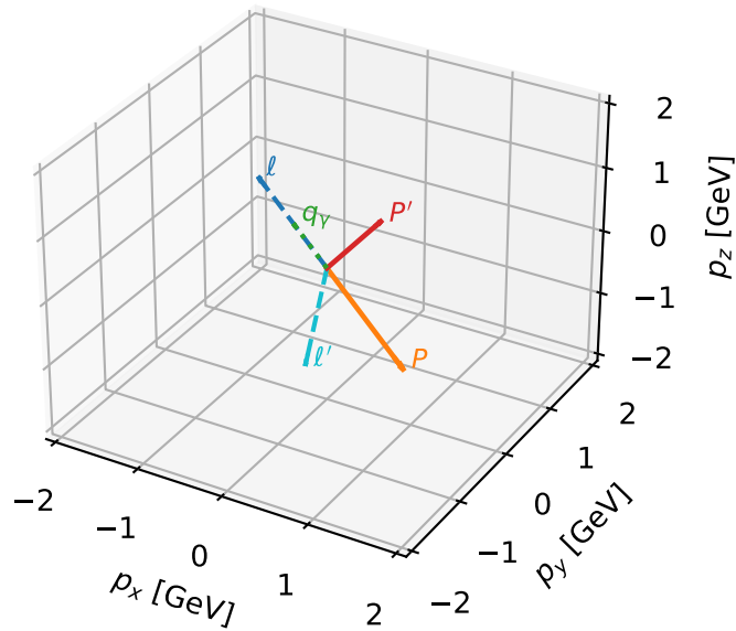
3D momenta
