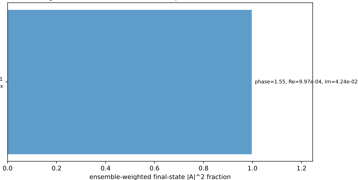
Leading initial-ensemble/final-state components (N=1, retained=99.7%)
