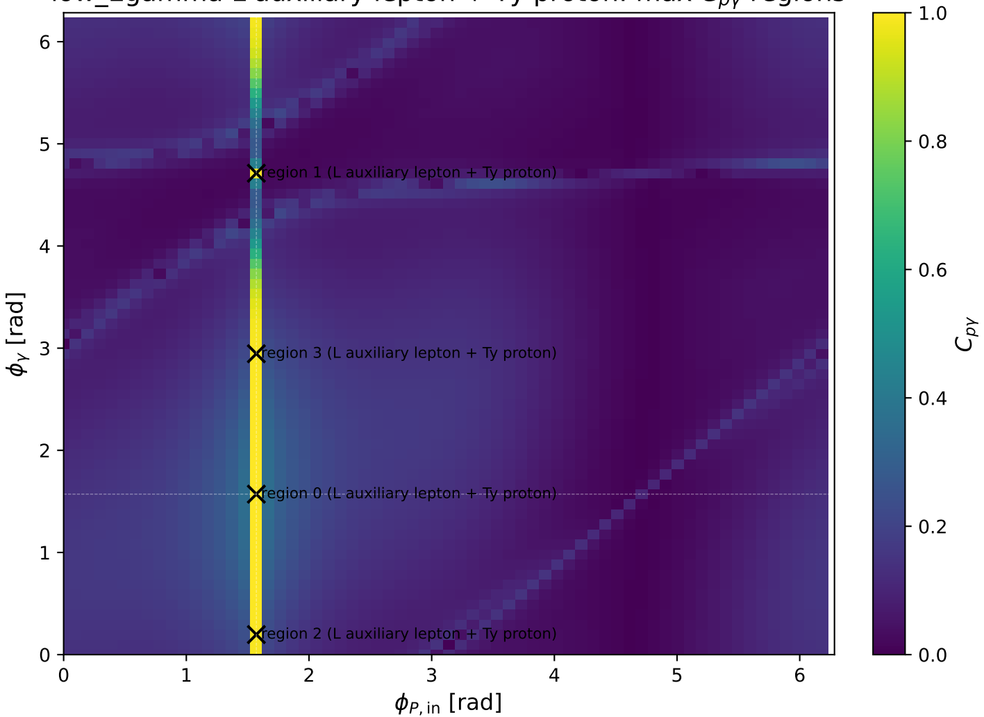
low_Egamma L auxiliary lepton + Ty proton: max C_{p\gamma} regions
