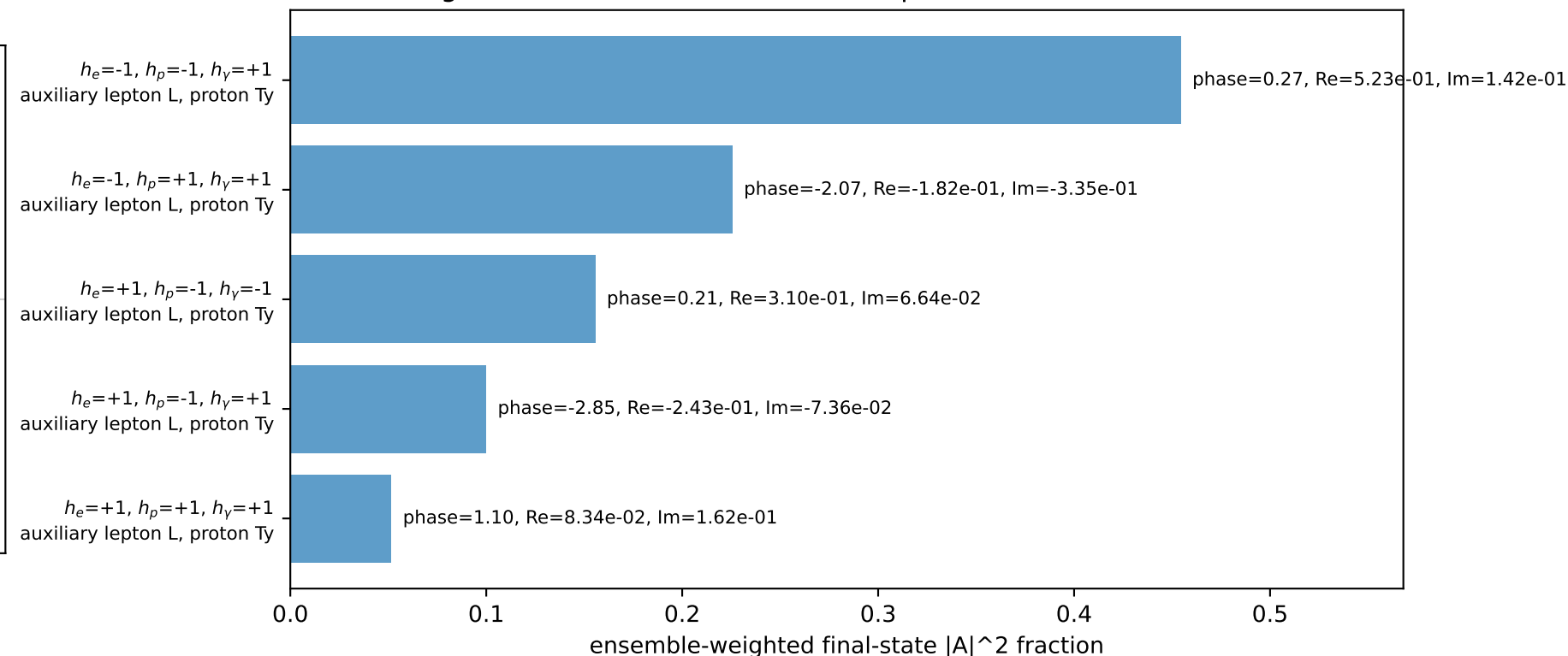
Leading initial-ensemble/final-state components (N=5, retained=98.7%)
