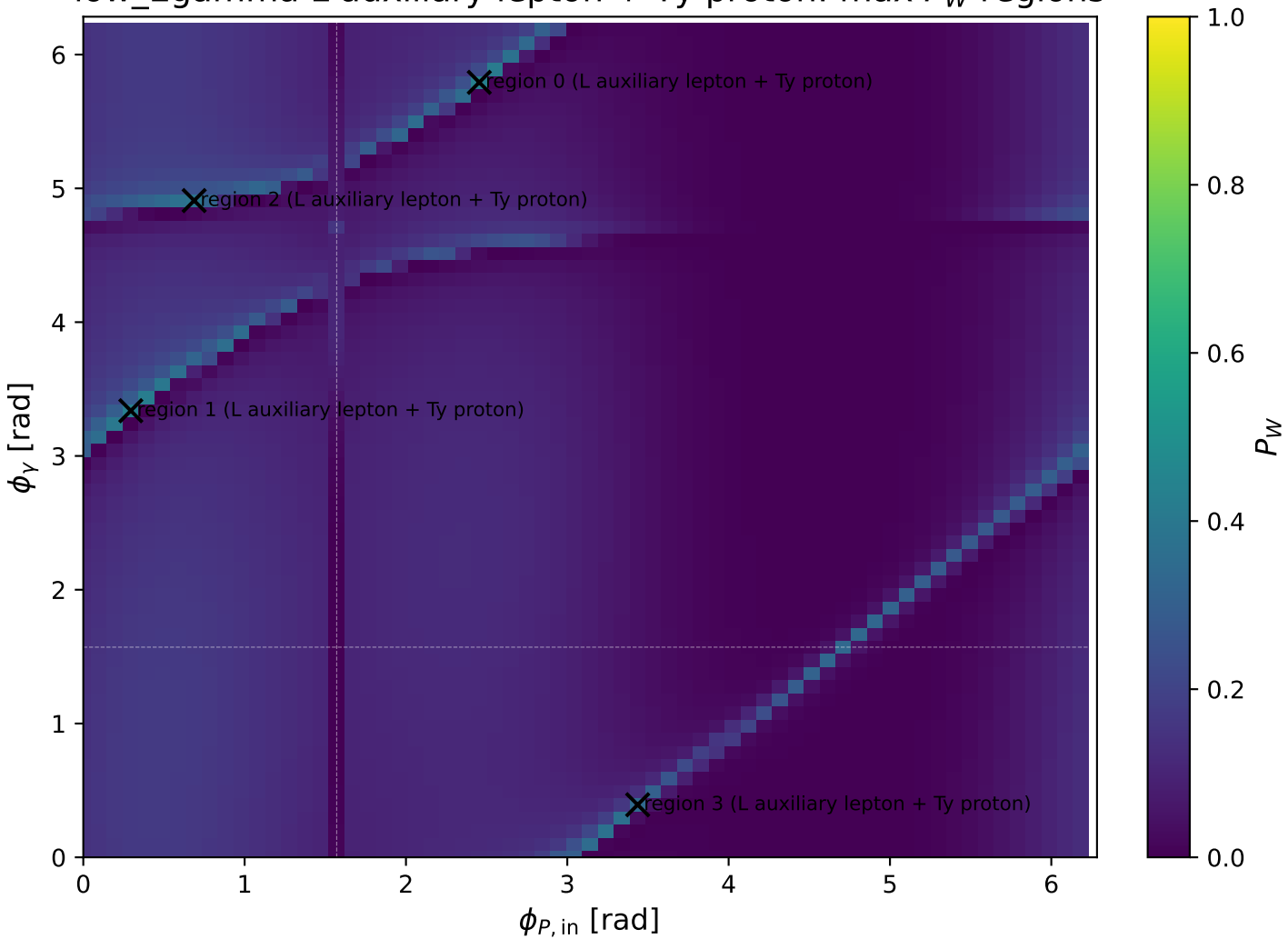
low_Egamma L auxiliary lepton + Ty proton: max P_W regions
