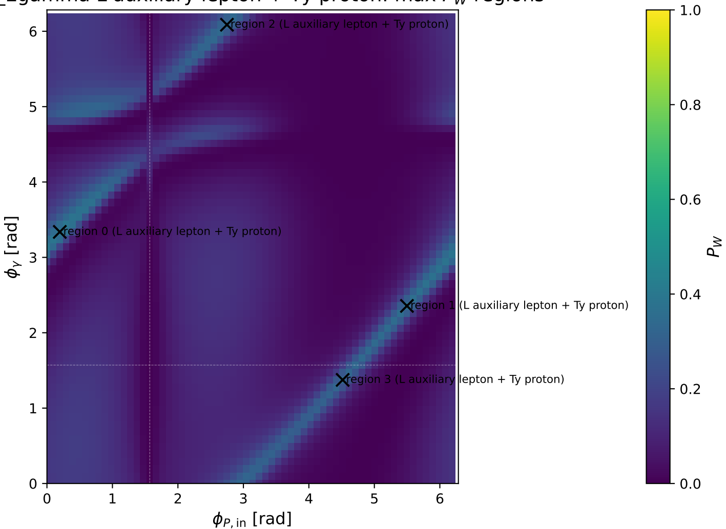
Egamma L auxiliary lepton + Ty proton: max P_W regions
