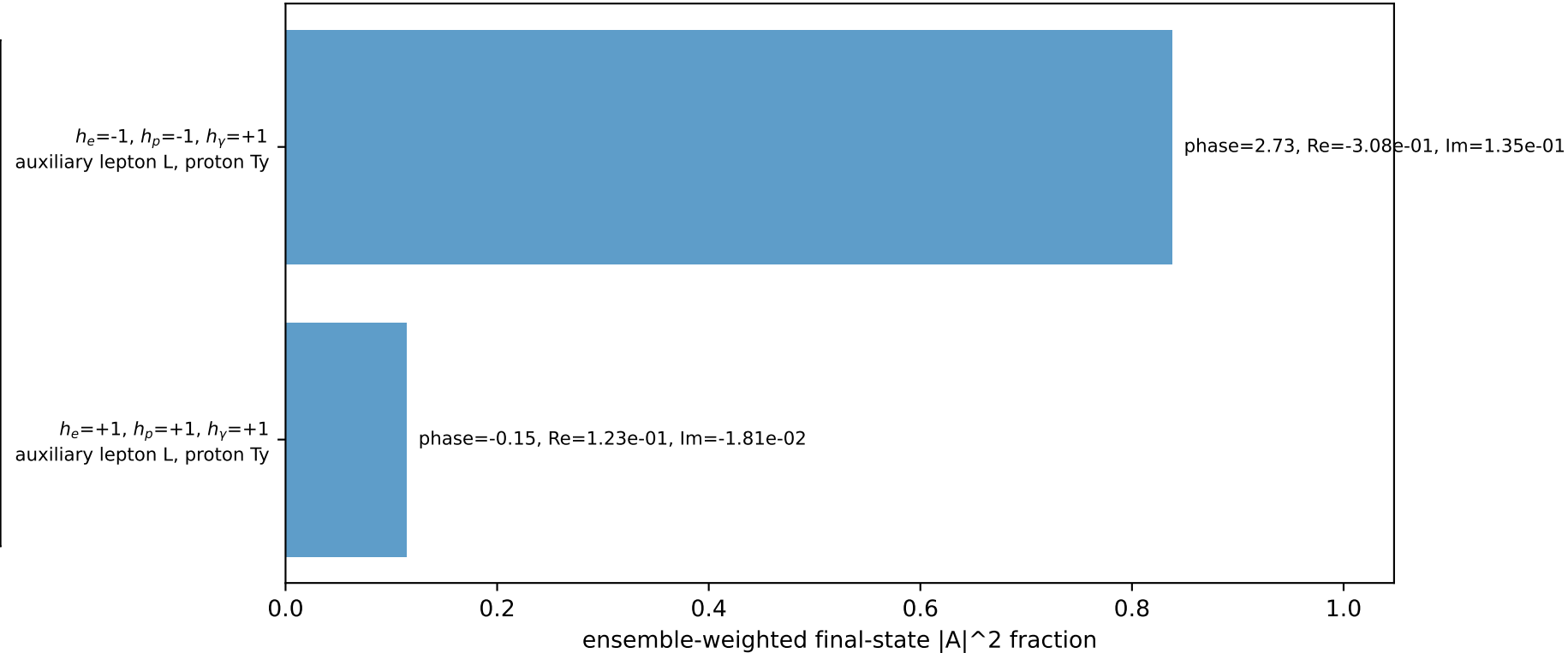
Leading initial-ensemble/final-state components (N=2, retained=95.3%)
