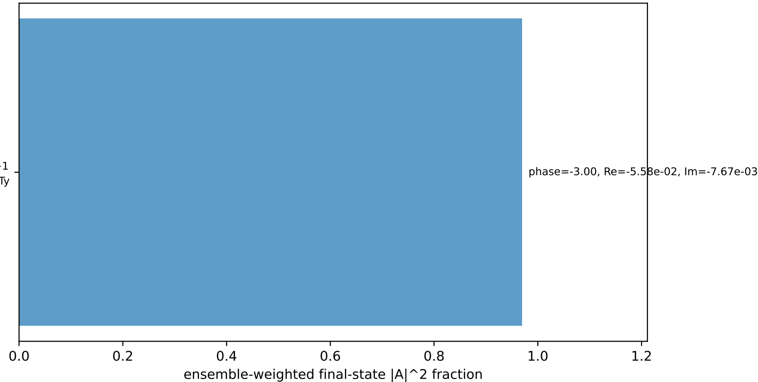
Leading initial-ensemble/final-state components (N=1, retained=96.9%)
