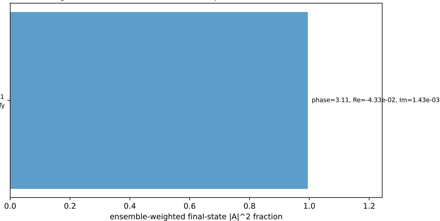
Leading initial-ensemble/final-state components (N=1, retained=99.5%)
