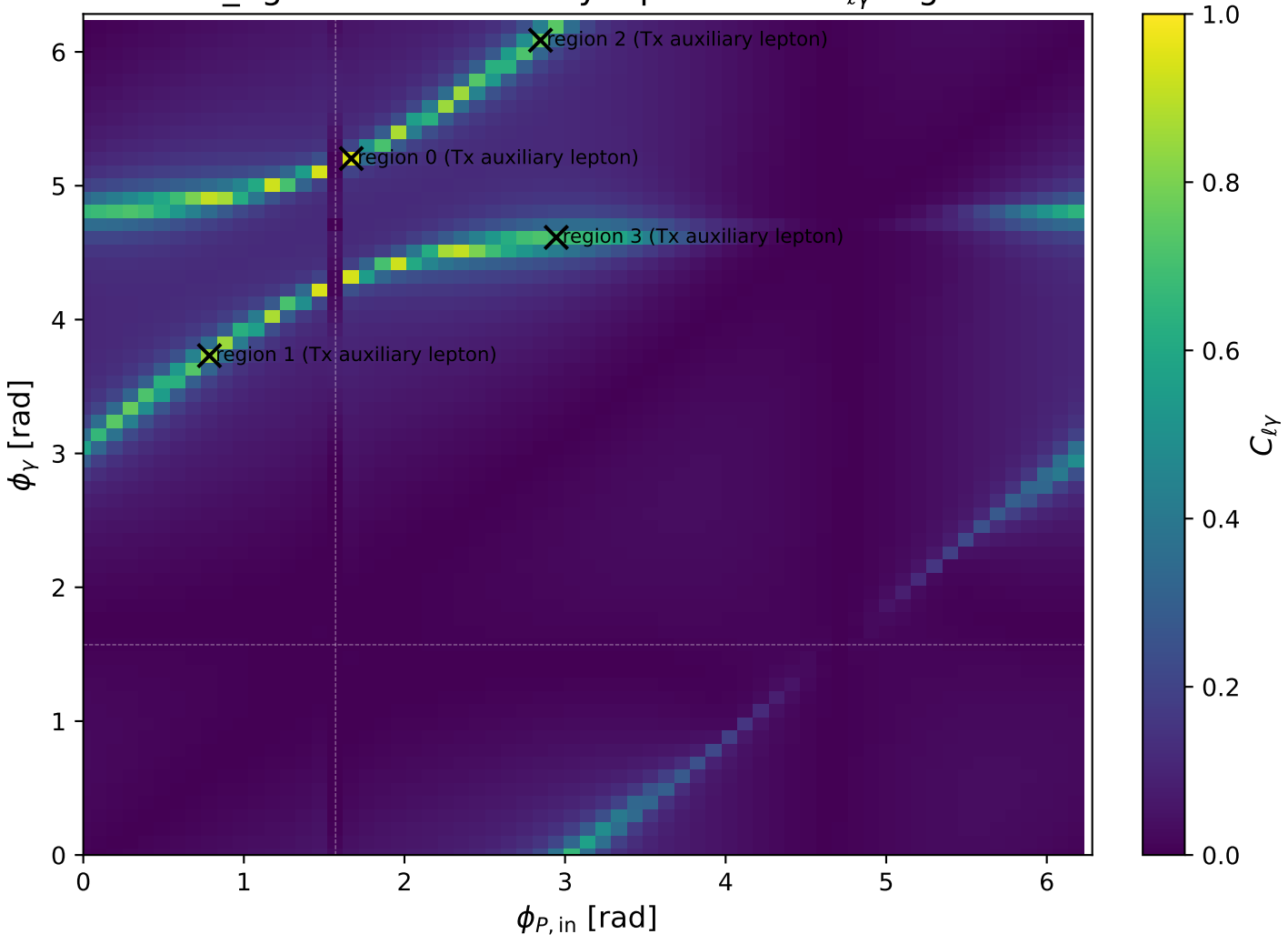
low_Egamma Tx auxiliary lepton: max C_{\ell\gamma} regions
