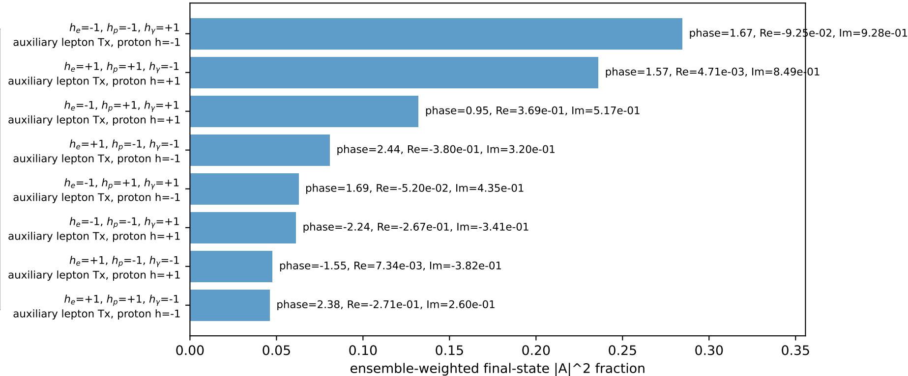
Leading initial-ensemble/final-state components (N=8, retained=95.1%)
