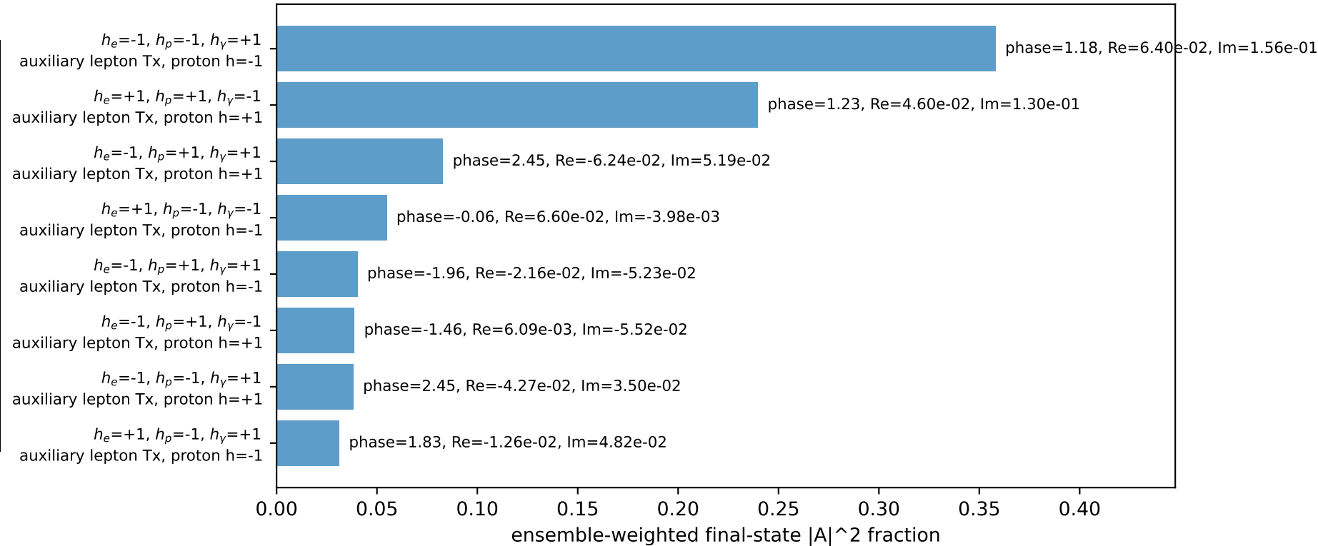
Leading initial-ensemble/final-state components (N=8, retained=88.4%)
