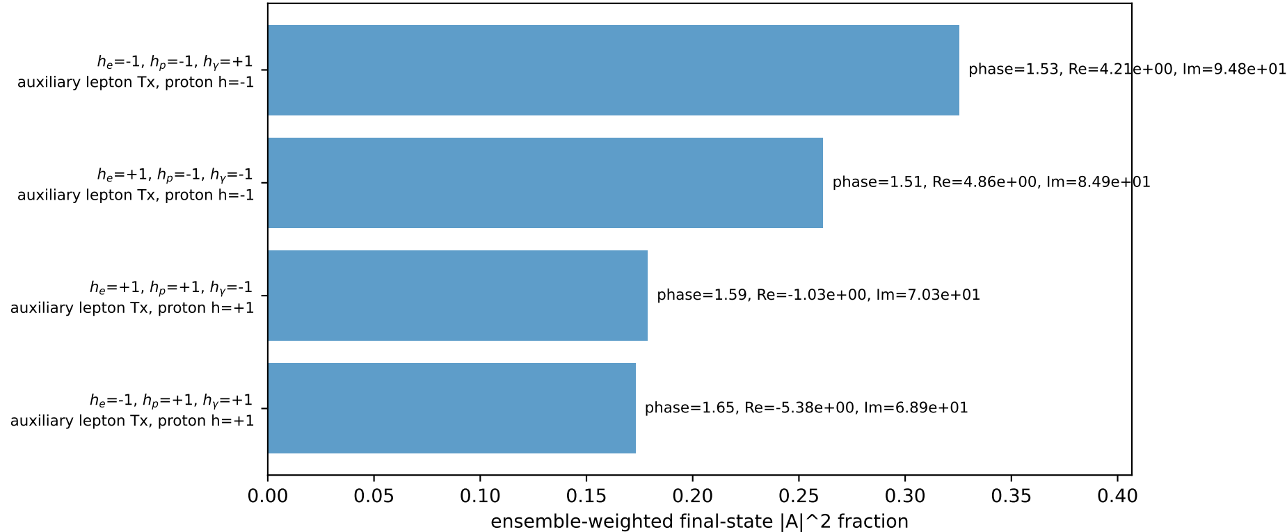
Leading initial-ensemble/final-state components (N=4, retained=93.8%)
