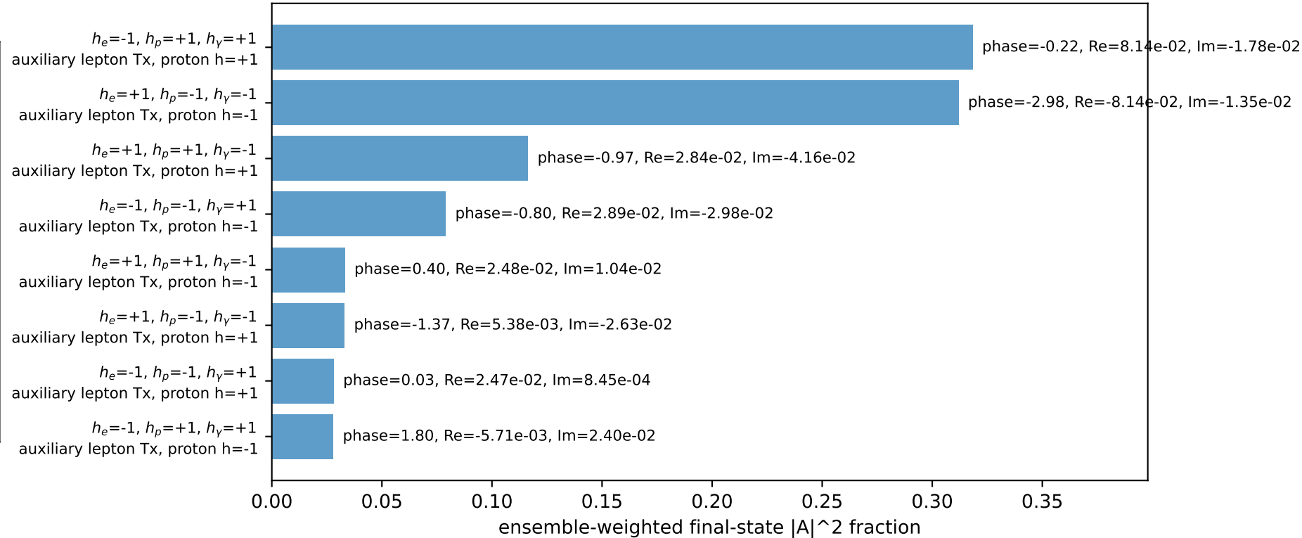
Leading initial-ensemble/final-state components (N=8, retained=94.8%)
