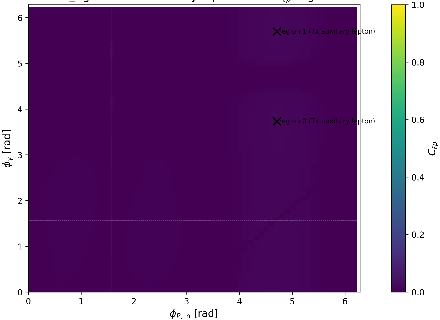
low_Egamma Tx auxiliary lepton: max C_{lp} regions
