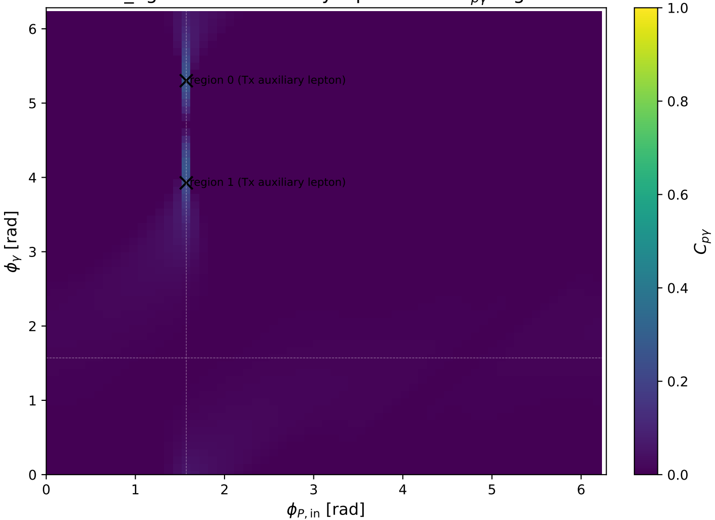
mid_Egamma Tx auxiliary lepton: max C_{p\gamma} regions
