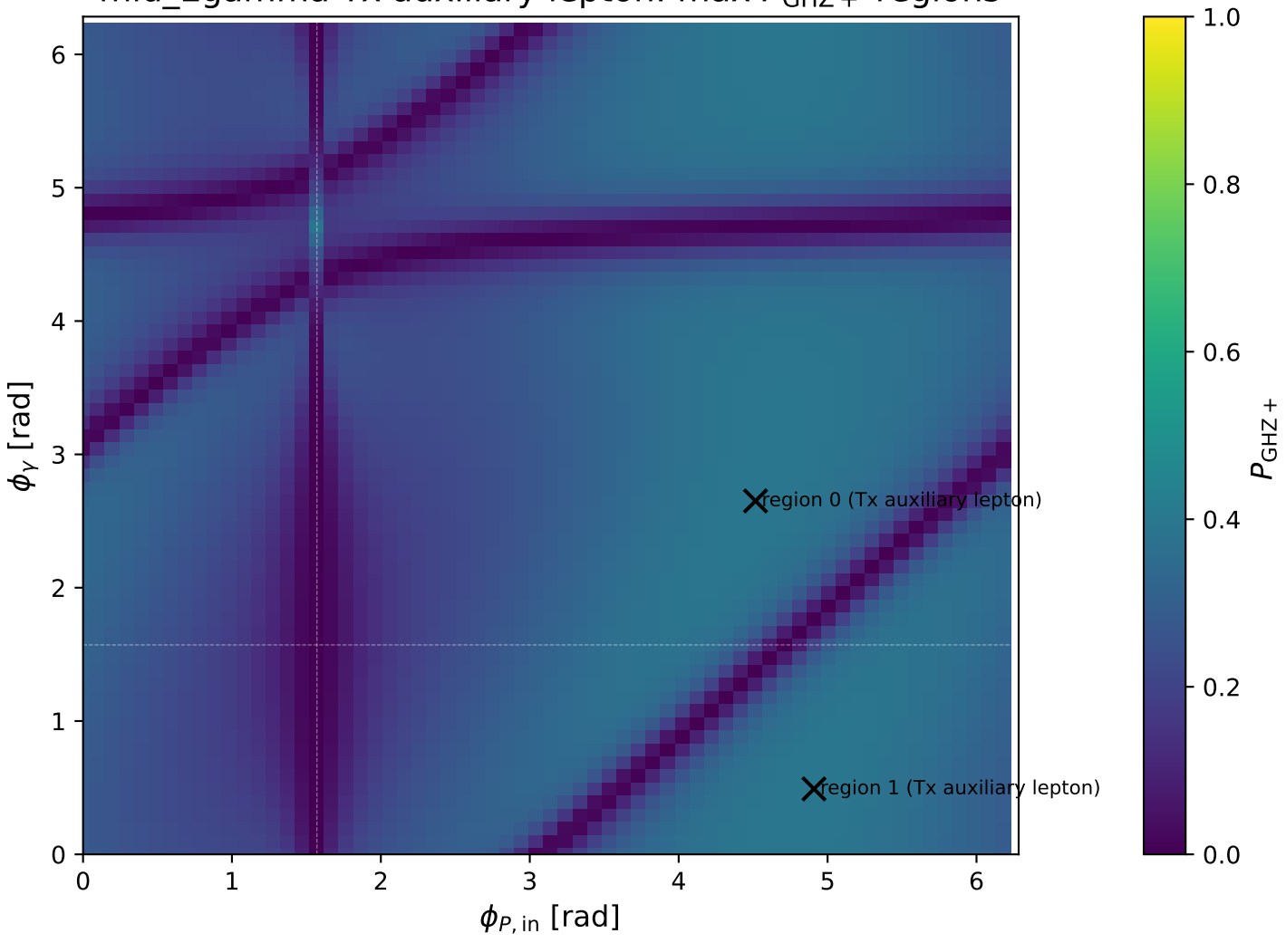
mid_Egamma Tx auxiliary lepton: max P_{\text{GHZ}+} regions
