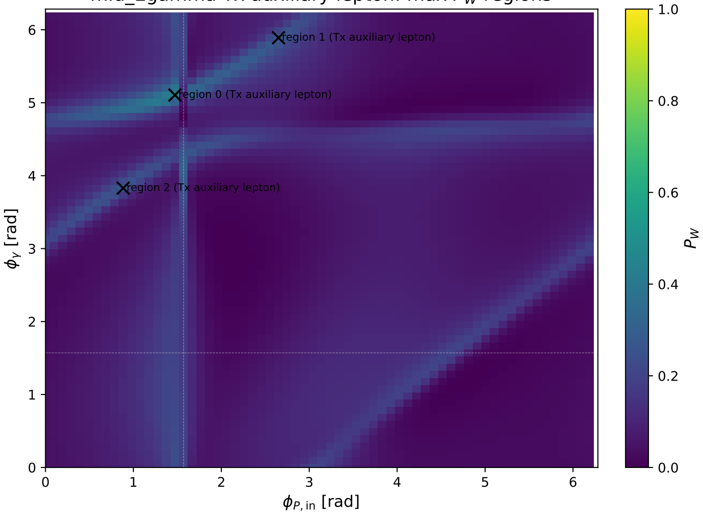
mid_Egamma Tx auxiliary lepton: max P_W regions
