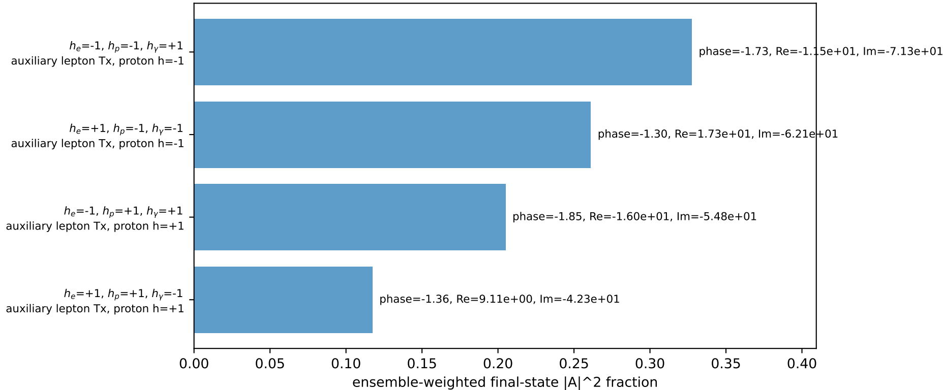
Leading initial-ensemble/final-state components (N=4, retained=91.1%)
