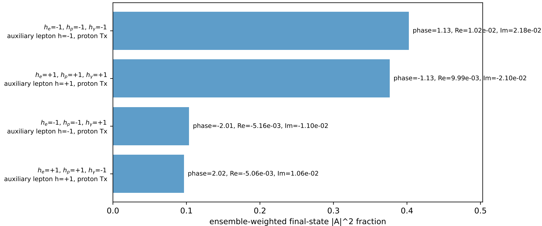
Leading initial-ensemble/final-state components (N=4, retained=97.8%)
