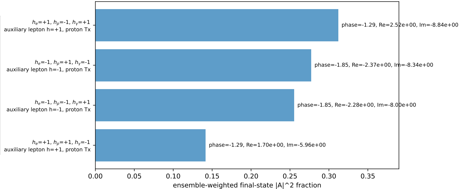
Leading initial-ensemble/final-state components (N=4, retained=98.6%)
