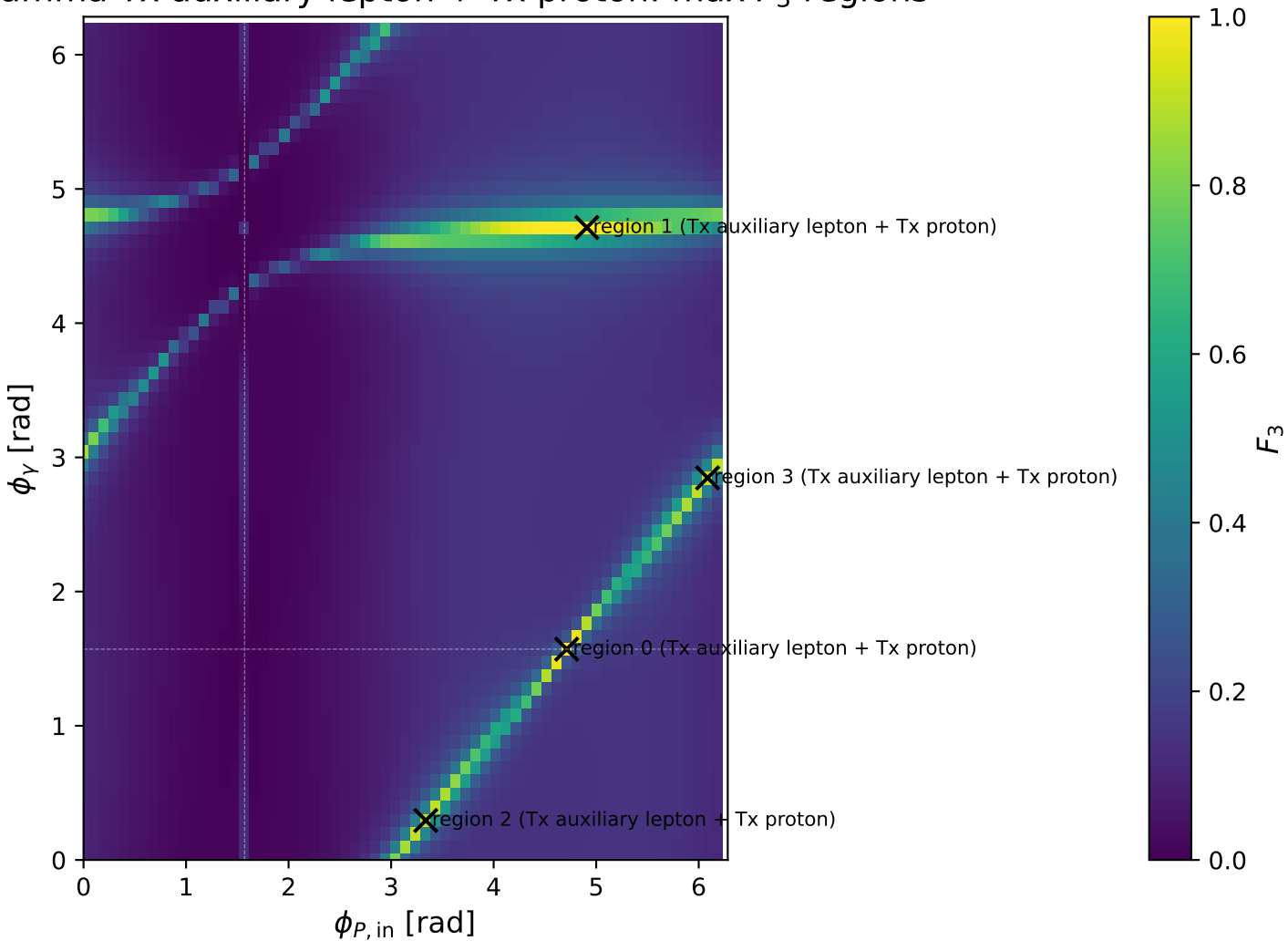
gamma Tx auxiliary lepton + Tx proton: max F_3 regions
