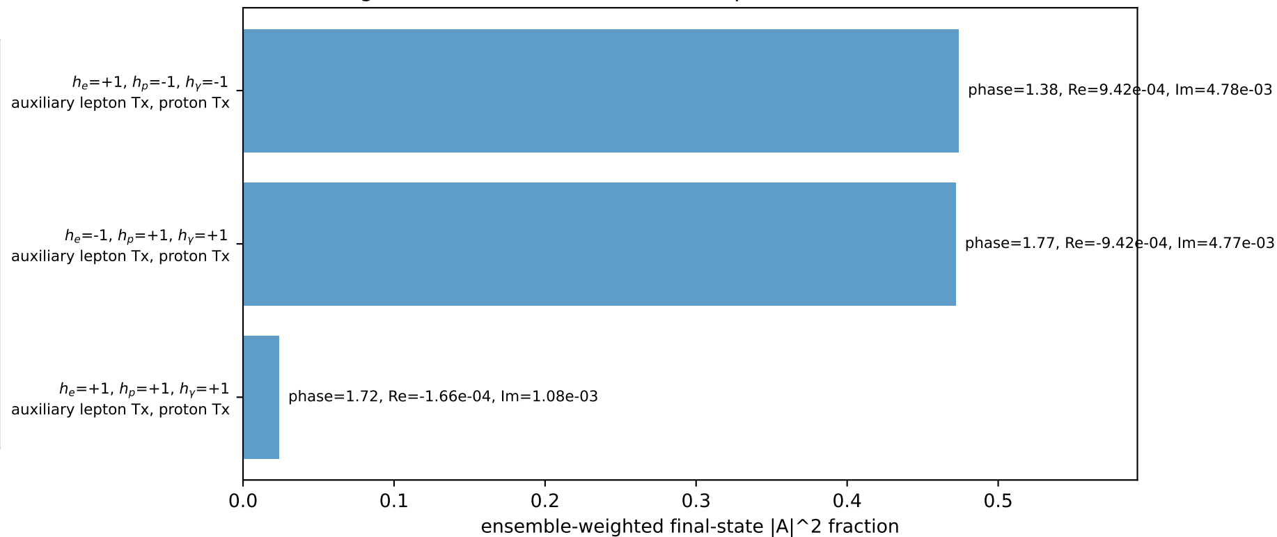
Leading initial-ensemble/final-state components (N=3, retained=96.9%)
