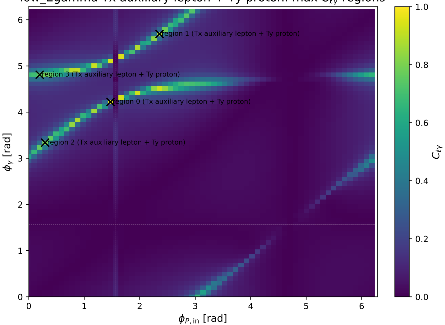
low_Egamma Tx auxiliary lepton + Ty proton: max C_{\ell\gamma} regions
