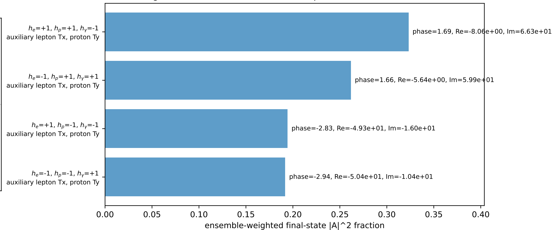
Leading initial-ensemble/final-state components (N=4, retained=97.1%)
