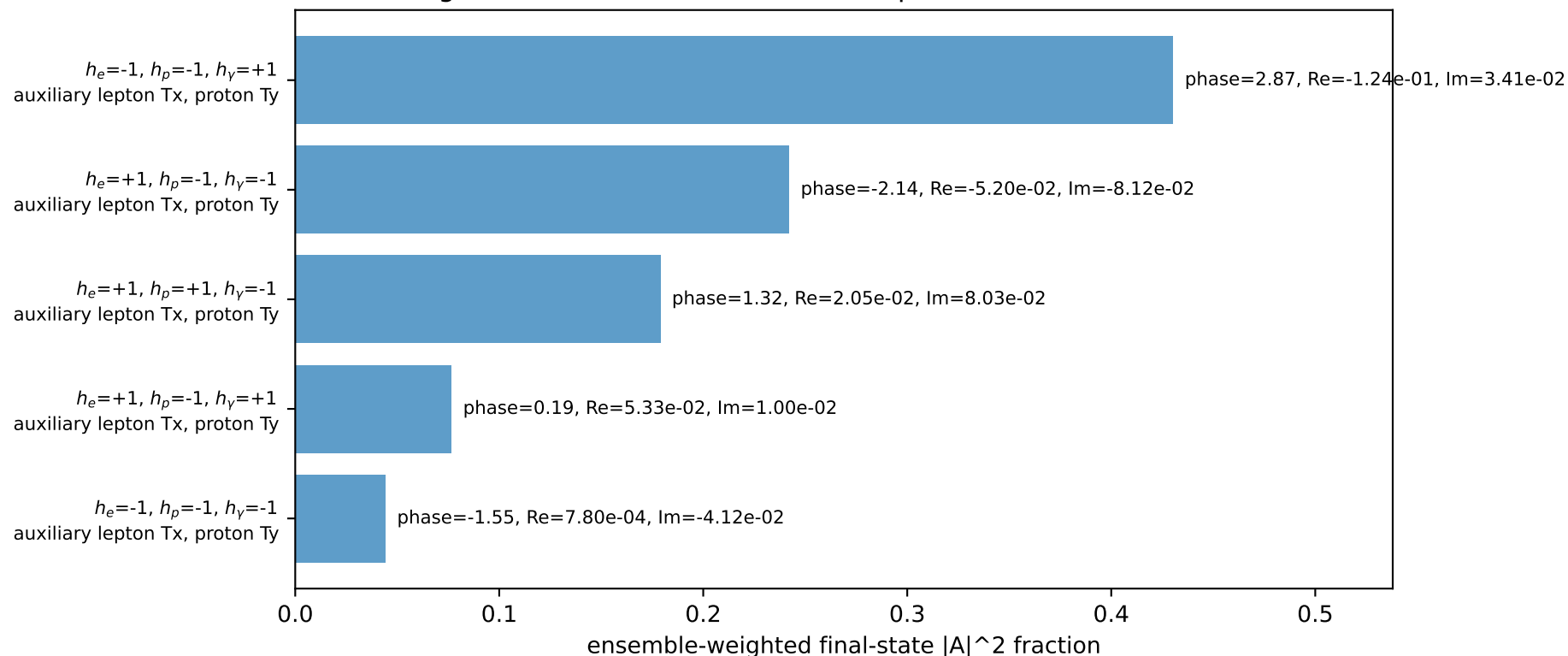
Leading initial-ensemble/final-state components (N=5, retained=97.2%)
