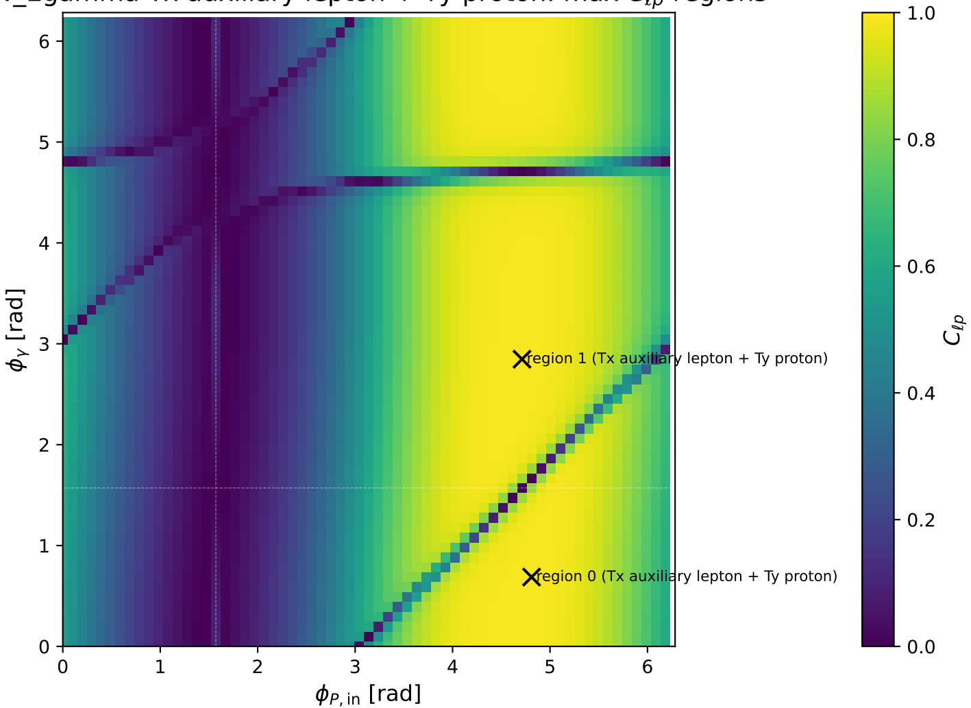
w_\Gamma Egamma Tx auxiliary lepton + Ty proton: max C_{lp} regions
