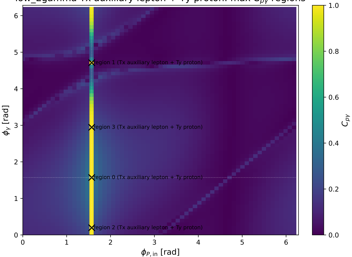
low_Egamma Tx auxiliary lepton + Ty proton: max C_{p\gamma} regions
